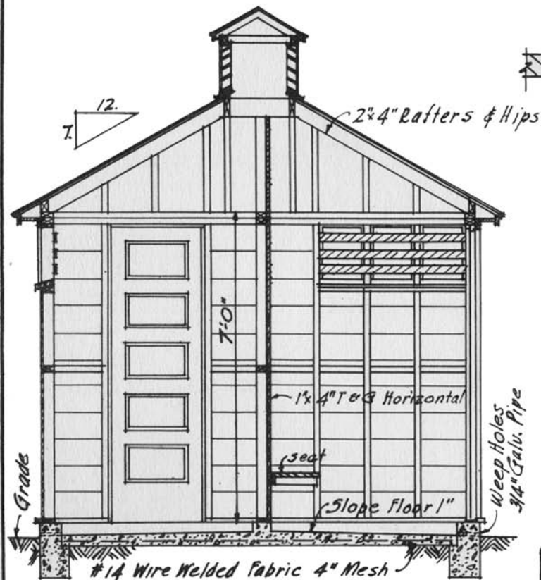
SECTION A-A Scale 3/8" = 1'-0"
