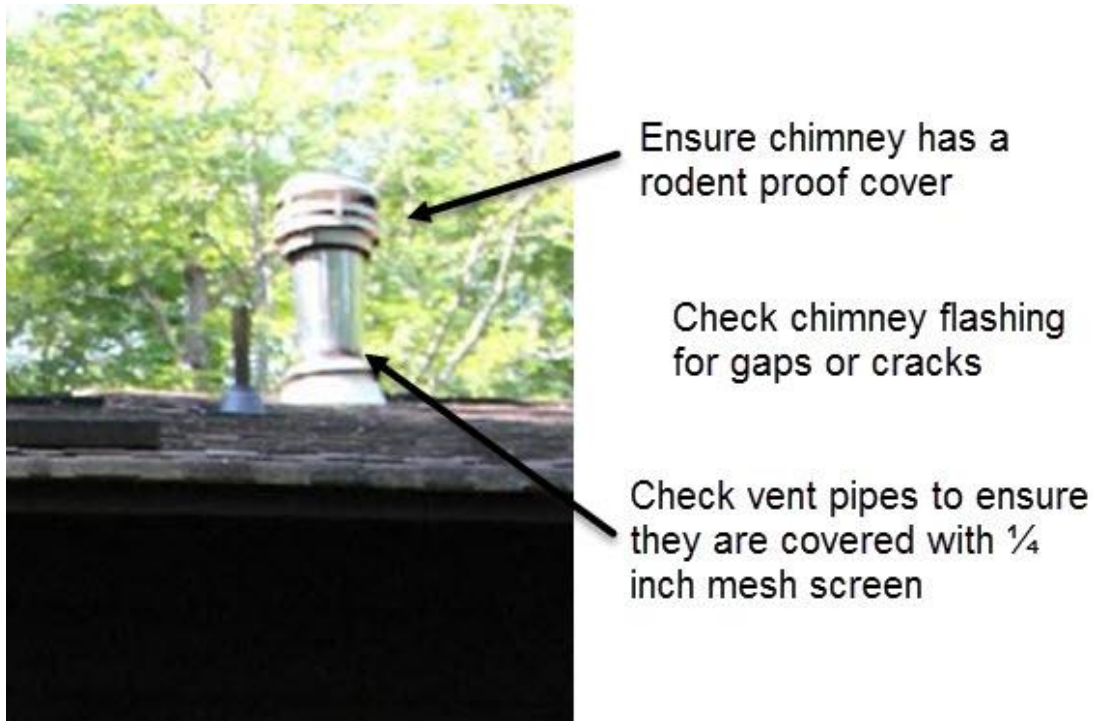
Figure 11: This properly installed chimney and vent pipe has a rodent proof cover. Evaluate the chimney and vent pipes on the roof to ensure that they are covered and flashing is tightly sealed to the roof. Also evaluate the roof for holes, gaps, or low points where water might pool and provide a water source to rodents. Figure credit: NPS Figure.
