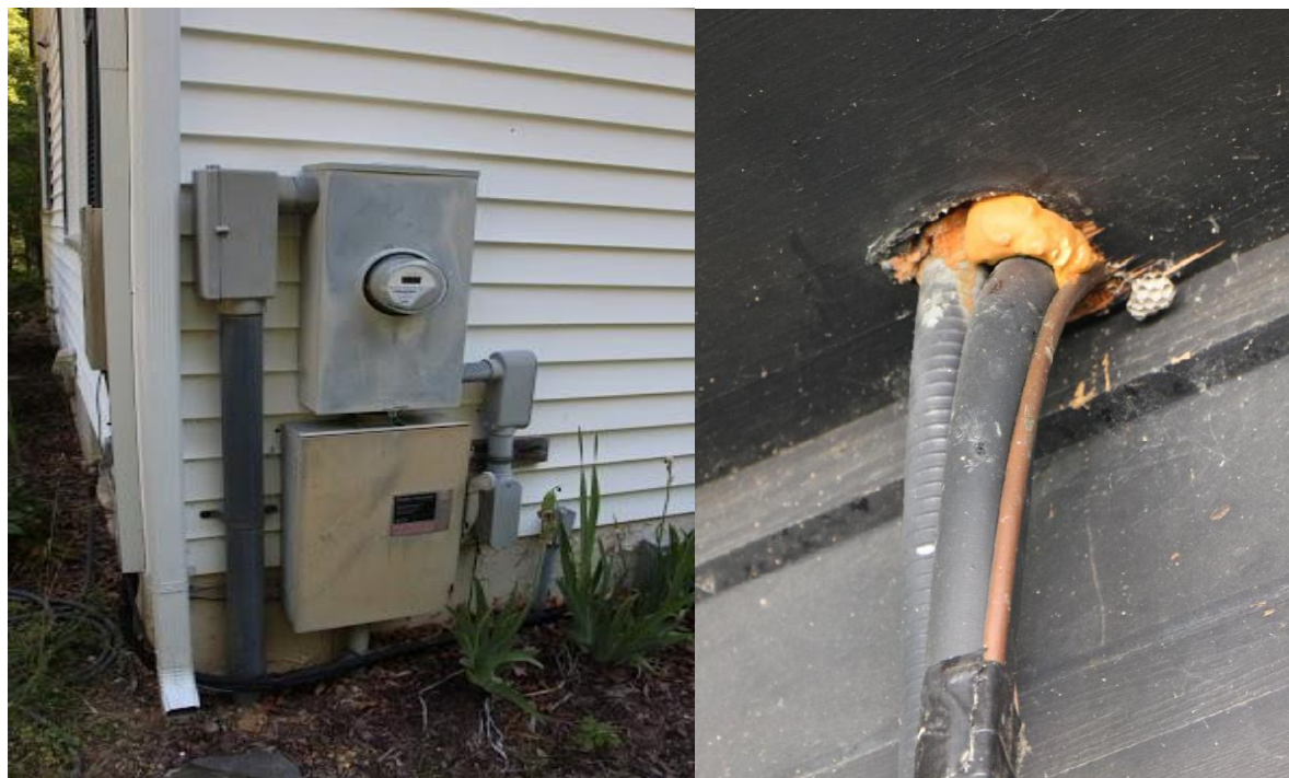
Figure 9 (left): Utility lines can leave gaps in the exterior of a building where they enter. Check for gaps or holes \frac{1}{4} " or larger around electrical, plumbing and gas lines entering the cabin, paying close attention to entry points that may be hidden behind service panels such as the ones shown in this picture. Seal up these openings to prevent rodent access. Figure credit: NPS Figure.
