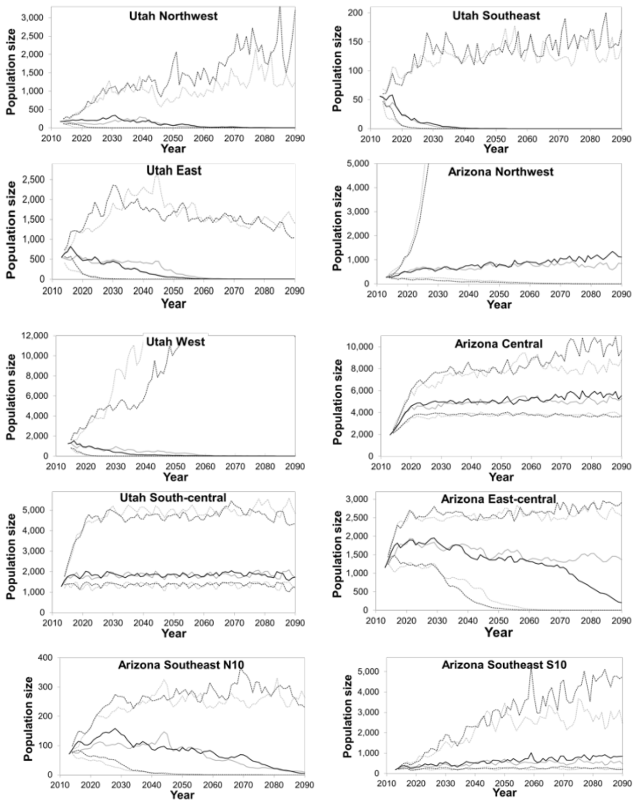
Figure 2.1. Pronghorn population projections to 2090 under high (RCP8.5; black lines) and lower (RCP4.5; grey lines) atmospheric CO 2 concentration scenarios for 16 pronghorn populations in the southwestern United States. Solid lines represent estimated median populations and dashed lines represent 2.5% and 97.5% credible intervals. See Table 2.2 for regression equations used in these models to project populations.
