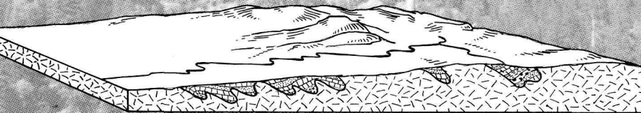
4 10 million years ago — a rolling surface of rounded low hills and broad valleys — including the primordial Yosemite Valley — is left. The Merced River meanders, 3,000 feet above its present position.
