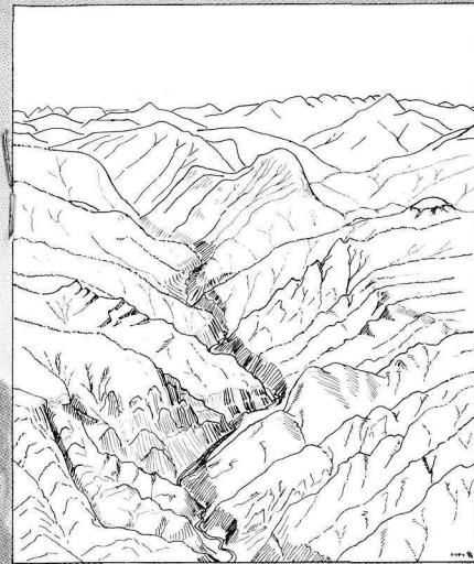
6 Further uplift again steepens the Merced River; it cuts a canyon within the mountain valley.
