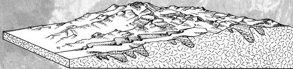
6 Further uplift again steepens the Merced River; it cuts a canyon within the mountain valley.
