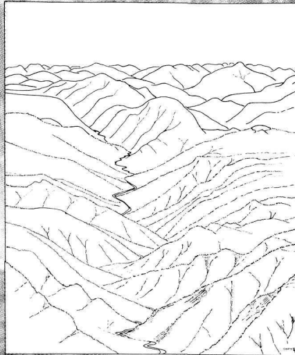
5 Renewed uplift of the Sierra Nevada steepens the Merced River; it cuts a mountain valley within the broad valley.
