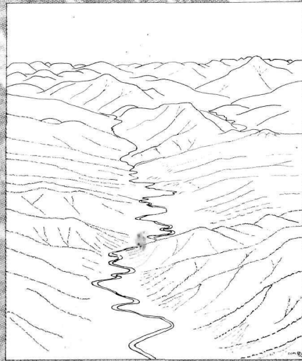
4 10 million years ago — a rolling surface of rounded low hills and broad valleys — including the primordial Yosemite Valley — is left. The Merced River meanders, 3,000 feet above its present position.
