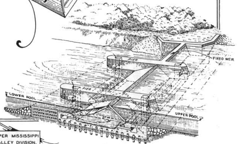
BEAR TRAP WEIR
