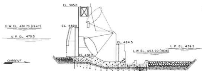
SECTION B-B
