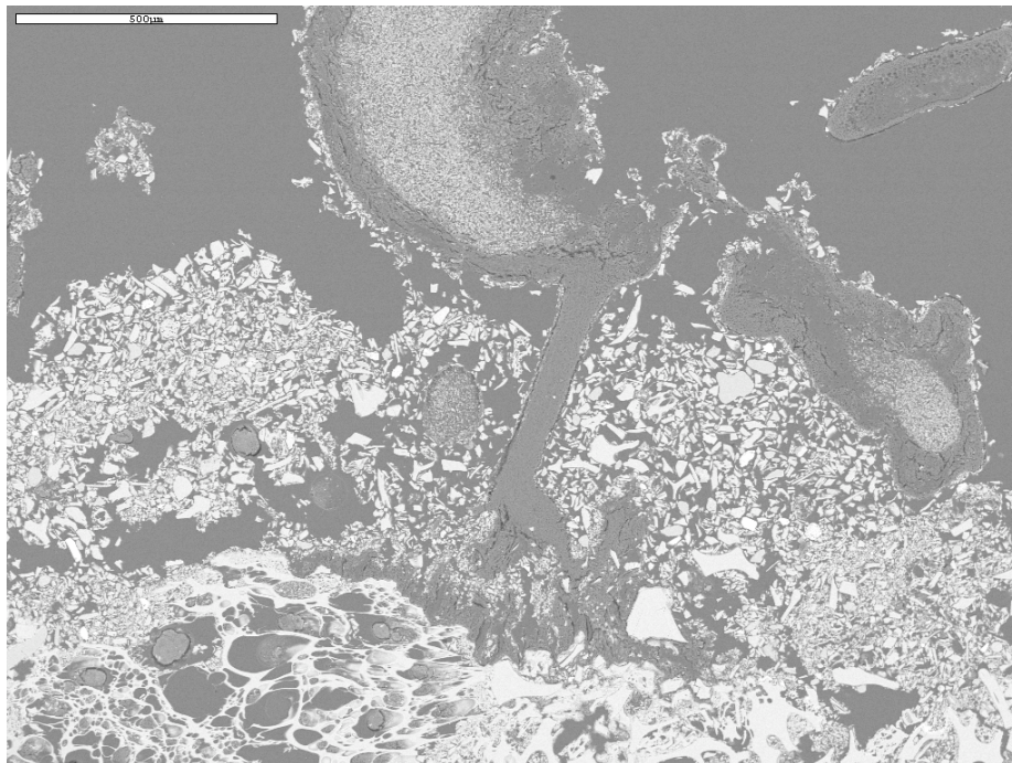
Figure 8. SEM backscatter image showing a lichen thallus on sedimented volcanic ash adhering to the canyon wall. The lichen is the dark mass at the top. The sedimented layer (middle zone) is over 500 \mu\text{m} thick and includes shards, ash, and crystal fragments embedded in a clay matrix. Lichen rhizines / hyphae (microfilaments) pervade the sedimented layer and help stabilize it. The canyon wall bedrock is the area with the large pumice at the bottom.
