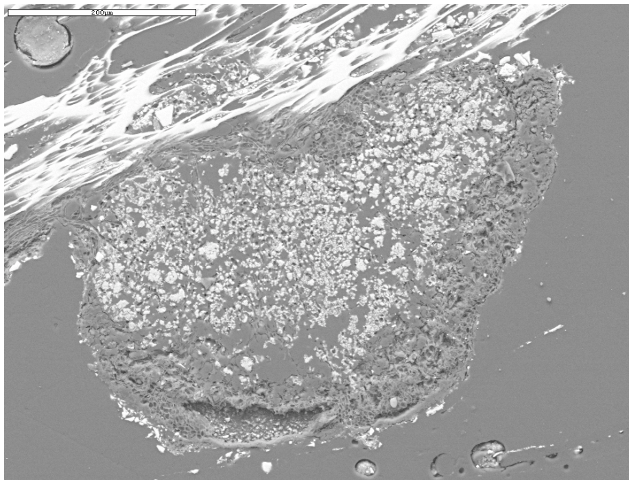
Figure 9. SEM backscatter image showing a lichen thallus growing directly on tuff on the canyon wall. The lichen is the dark mass with the cellular structure. Light gray crystals of weddellite (calcium oxalate) fill the thallus. Microfilaments invade the long-tube pumice vesicles of the bedrock tuff at the top of the photo.
