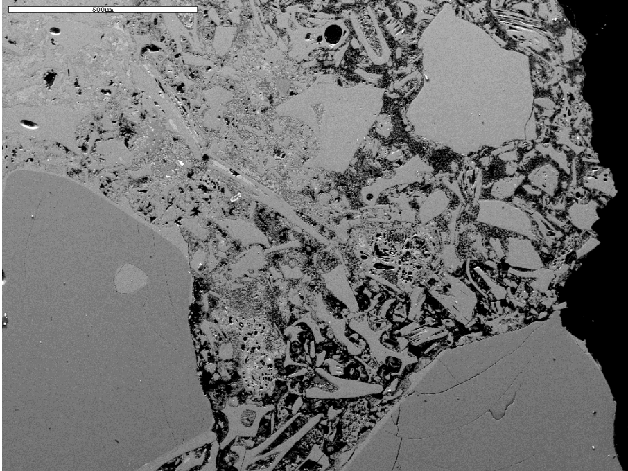
Figure 12. SEM backscatter image of case hardened tuff with alteration typical of Types 3 to 5. At the sample surface (right), the larger glass shards are moderately scalloped and unfilled pore spaces still account for 30-40% of the sample volume. Moving left, there is more dissolution and replacement of the original material and pore space is reduced to < 20%. Opal is the dominant filling material; other filling materials include sepiolite and intergrown calcite and opal. At the far left, open pore space is less than 5% at a depth of approximately 1.30mm.
