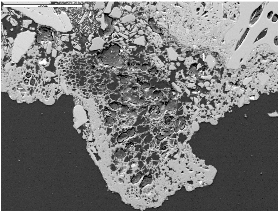
Figure 13. SEM backscatter image showing pseudomorph of lichen thallus replaced by opal in a case hardened surface; delicate cellular structure of the lichen is preserved by the mineralization. The lichen is attached to tuff bedrock where most of the fine ash in the matrix is replaced by intergrown opal and clay. Small bright white areas are trace barite.
