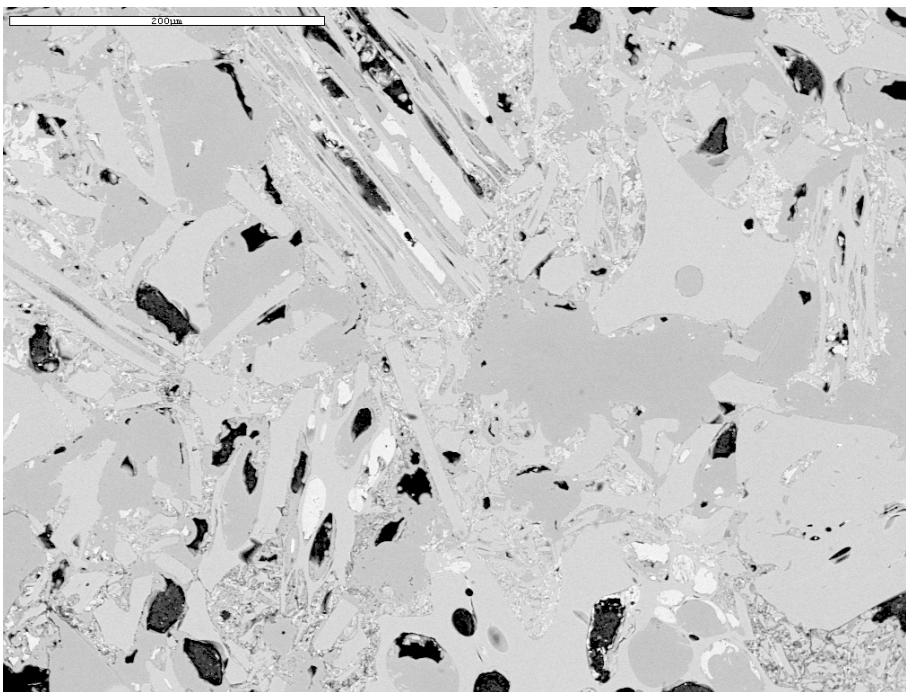
Figure 16. SEM backscatter image for the inner band of alteration in Type 7 case hardened tuff. Large glassy shards (light gray) show few delicate cusped structures due to dissolution. The shards are thoroughly cemented by massive opal (medium gray), calcite (white), and sepiolite (small mottled dark gray areas). All of the fine matrix ash and most of the original pore space have been replaced by mineralization. The few remaining pores are shown in black. Image analysis yields the following proportions: 49.2% glass shards, 43% opal, 4.3% calcite, trace sepiolite, and 3.5% porosity.
