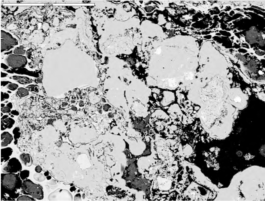
Figure 15. SEM backscatter image for the outer band of alteration in Type 7 case hardened tuff. Volcanic ash in the tuff matrix is replaced by thick, massive bands of opal (medium gray) and finely intergrown opal and clays (mottled appearance). Some larger glassy pyroclasts (vesicular pumice and 100- \mu m-wide equant clast in the upper left quadrant) survived alteration, but show moderate to severe effects of dissolution at their margins. There are thin rinds of opal pseudomorphs replacing pumice vesicles in the center left part of the image.
