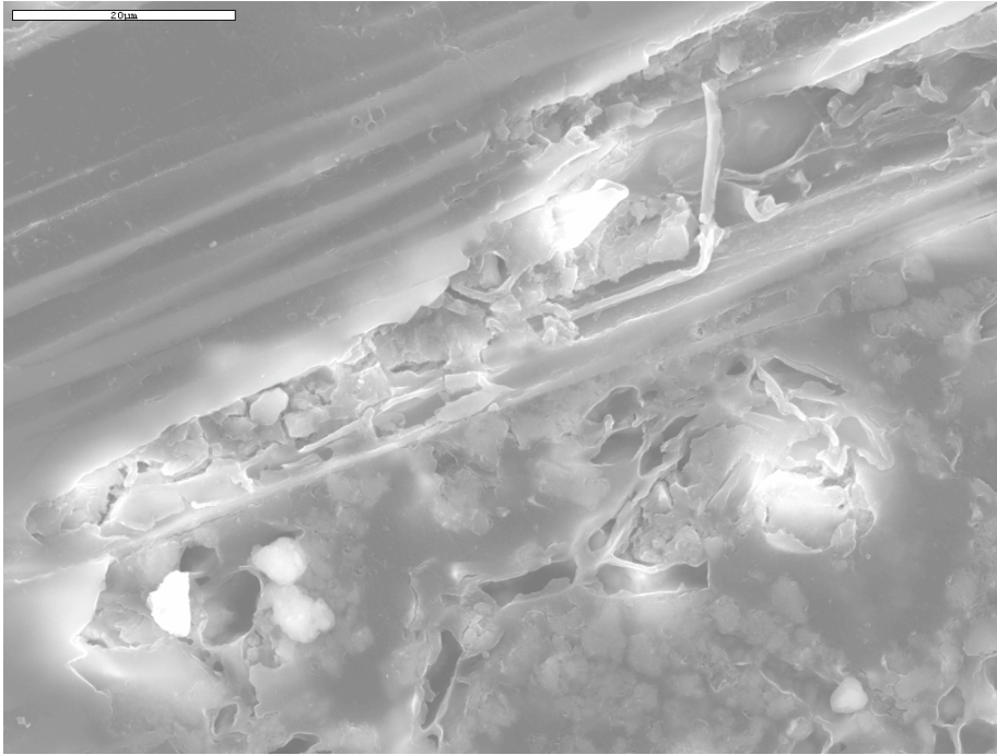
Figure 10. SEM secondary electron image showing dissolution of pumice vesicle walls in contact with lichen hyphae. The tubular pumice (extending from lower left to upper right) has scalloped edges. Lichen (lower right) is in contact with the pumice and hyphal filaments invade the large open vesicle (upper right).
