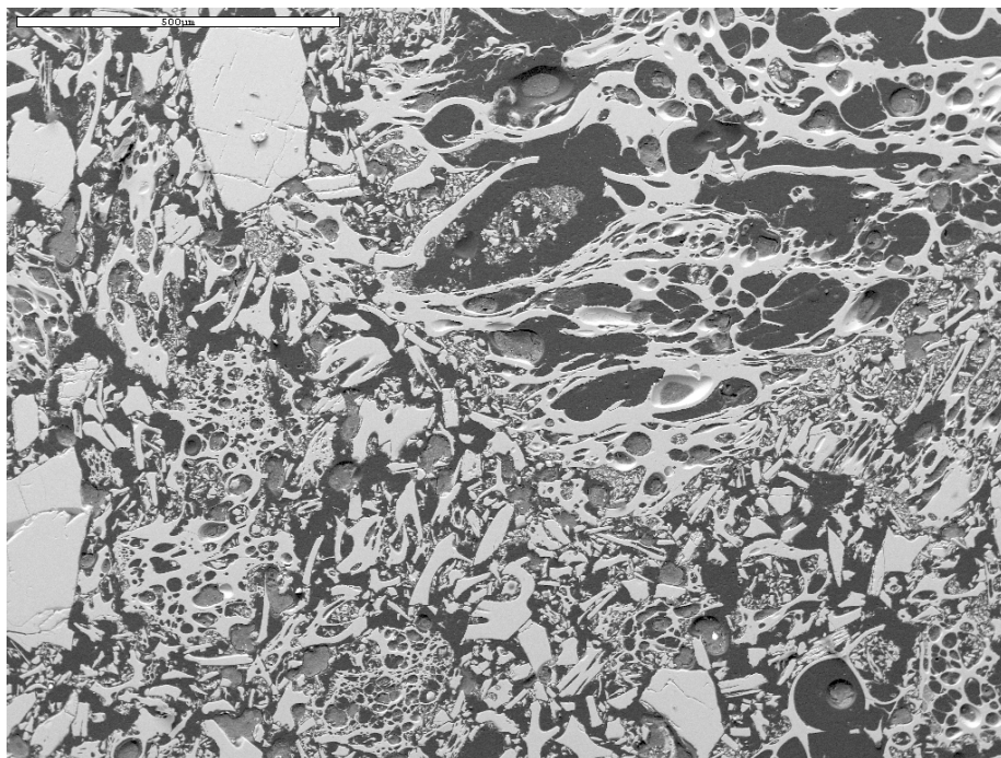
Figure 11. SEM backscatter image of canyon wall tuff bedrock with Type 1 to 2 alteration. The tuff has undergone minimal alteration and lacks cementation by secondary minerals. The tuff contains abundant vitric ash in the groundmass, and delicate shard and pumice lapilli structures are well preserved. The porosity of the tuff is 40 to 50%.
