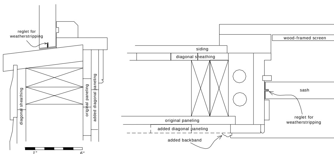
Figure 53 Section and plan of typical window opening; internal framing details conjectural. (T. Jones, NPS-SERO-CRS, 2002)
