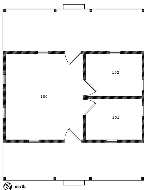
Figure 9 Probable plan of Guthrie-Ogilvie House as originally constructed. (T. Jones, NPS-SERO-CR, 2003)
