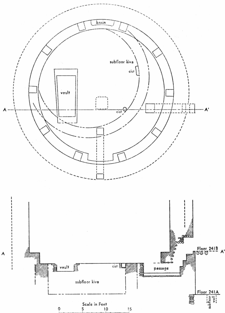
FIG. 18.—Kiva D with subfloor features and cross section.
