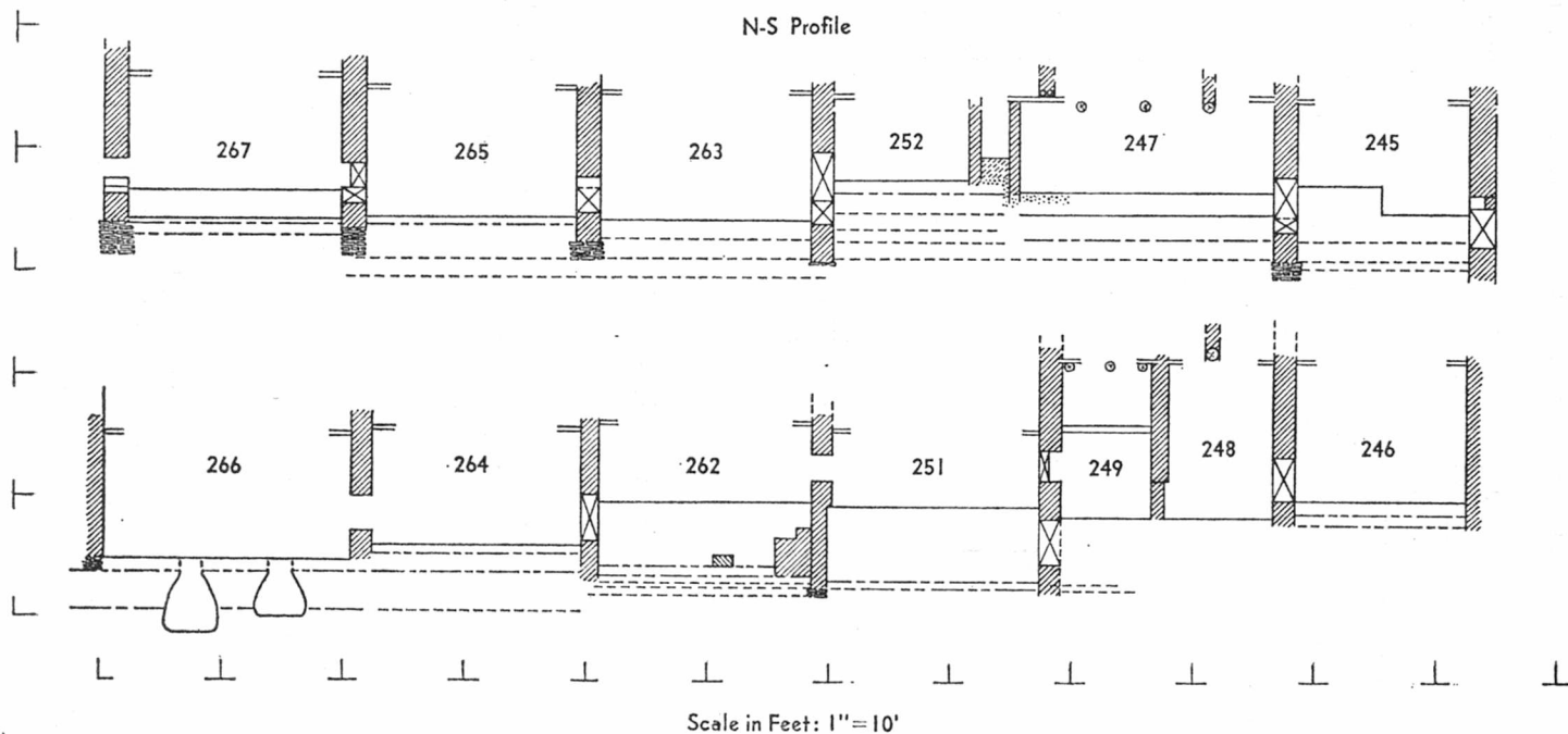
FIG. 8.—North-south profile, Rooms 266-267 through Rooms 245-246, showing earlier floor levels.
