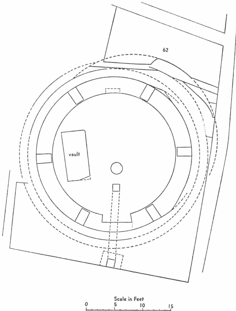
FIG. 19.—Kiva G, of second-type masonry was twice remodeled.
