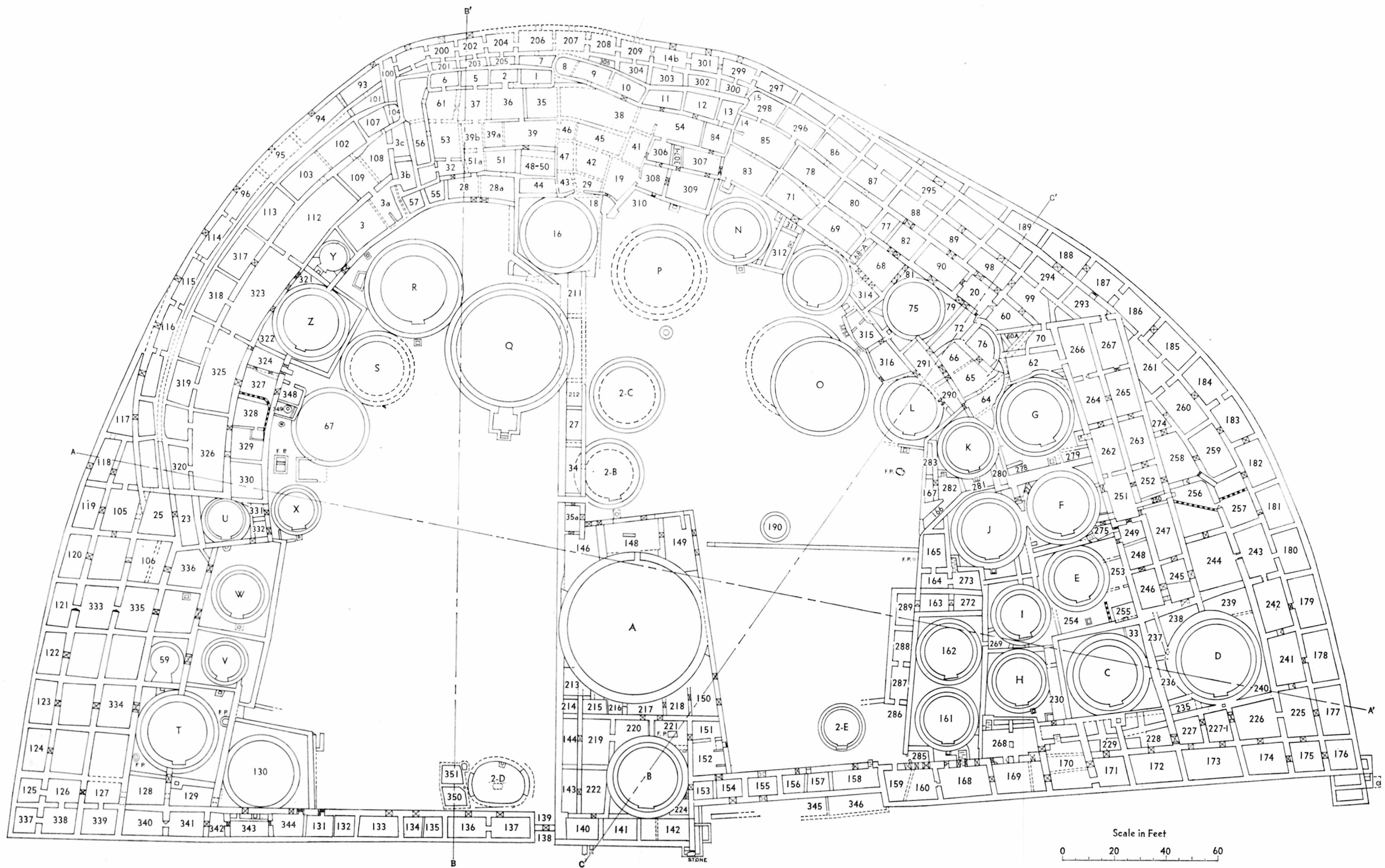
FIG. 2.—Ground plan of Pueblo Bonito with cross sections A-A', B-B', and C-C'. (From the original survey of Oscar B. Walsh, 1925.)
