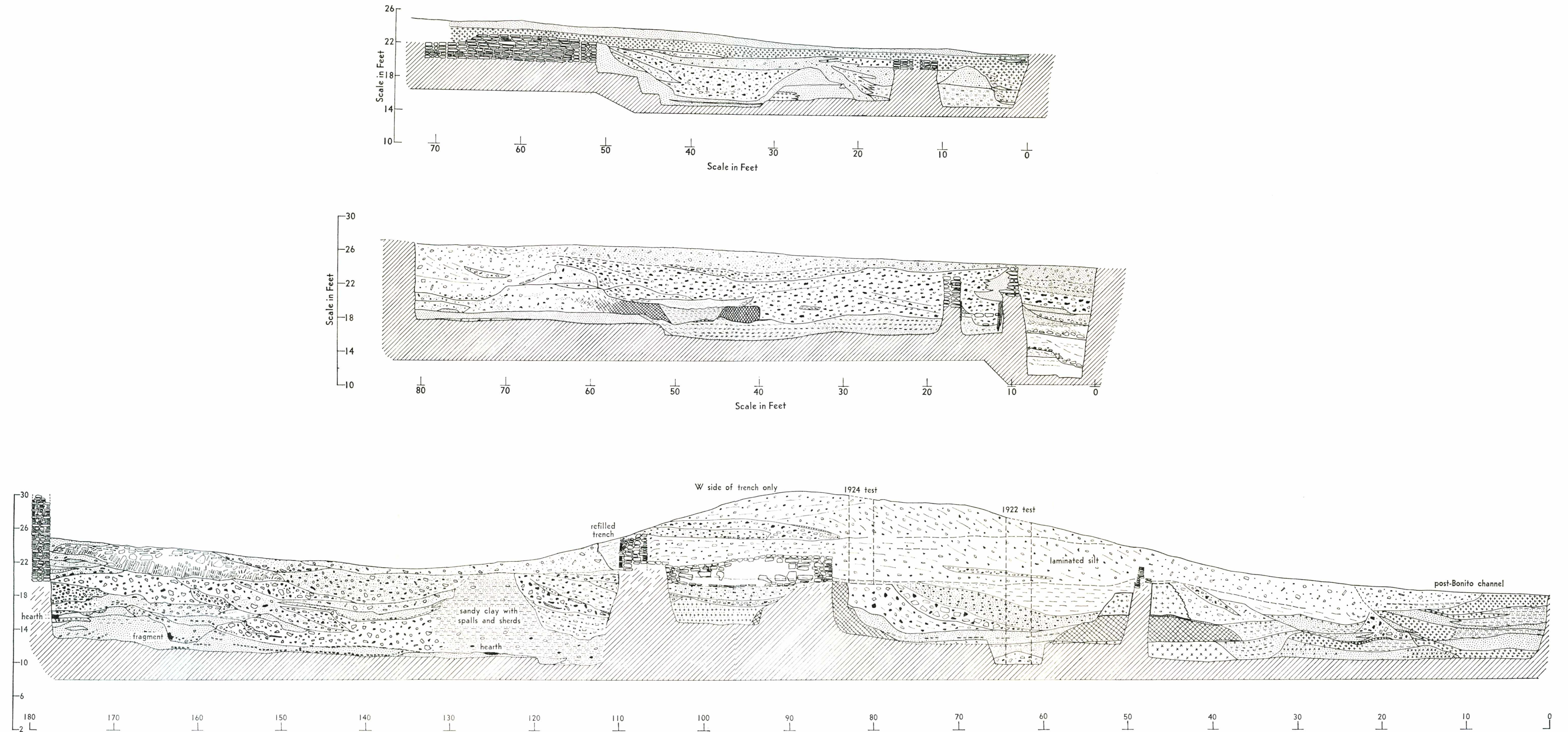
FIG. 24.—The “Far East Trench” (upper); the “Middle Trench”; and the “East Mound Trench” from the post-Bonito channel to the foundations of Room 171.
