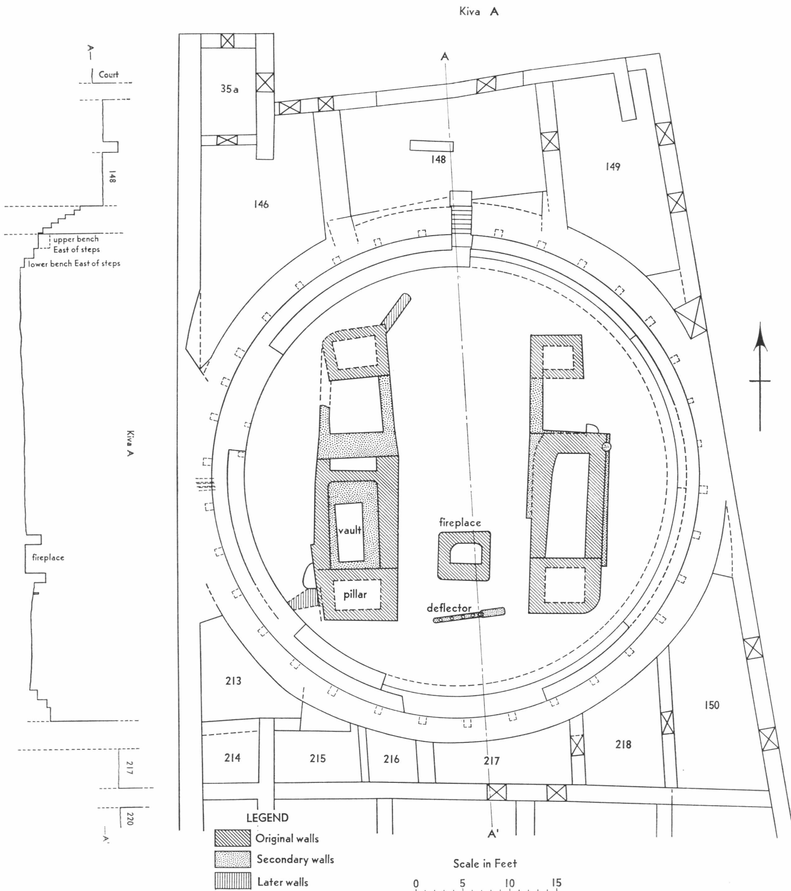
FIG. 16.—Great Kiva A with cross section A-A'.
