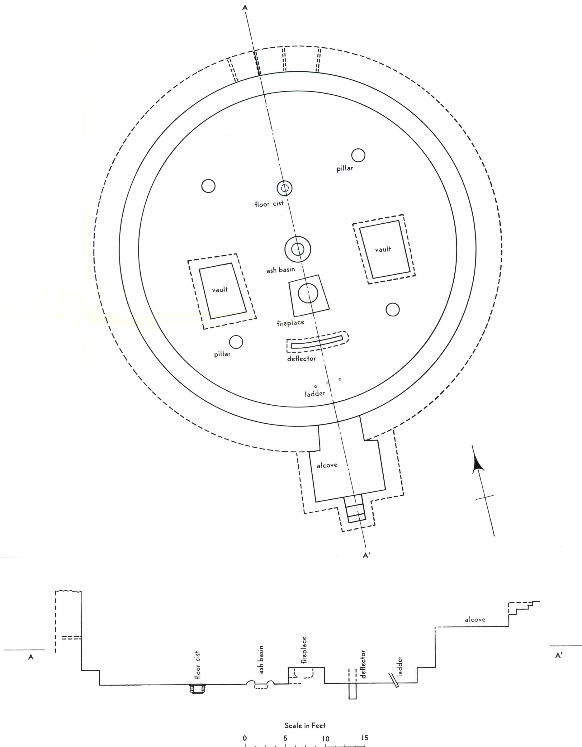
FIG. 17.—Great Kiva Q and cross section A-A'.
