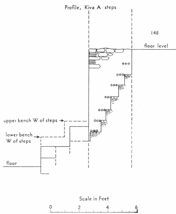
FIG. 16a.—Profile of Kiva A stairway from latest floor to Room 148.
