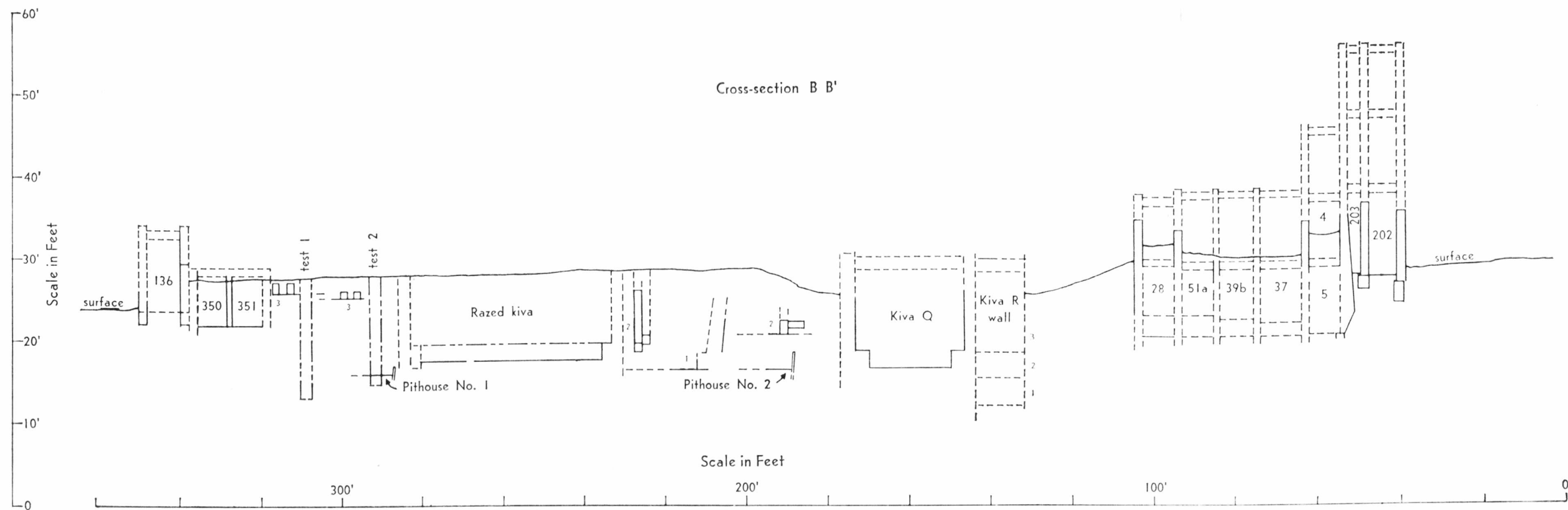
FIG. 14.—Cross section B-B' from Room 202 to surface outside Room 136.
