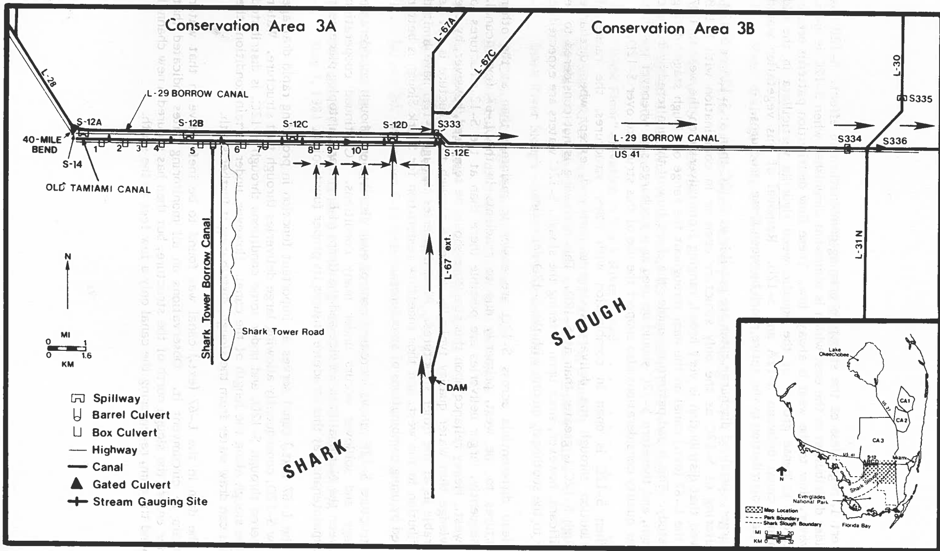
Figure 13. Northward flow out of the Park through the S-12 distribution system, May 7, 1981.
