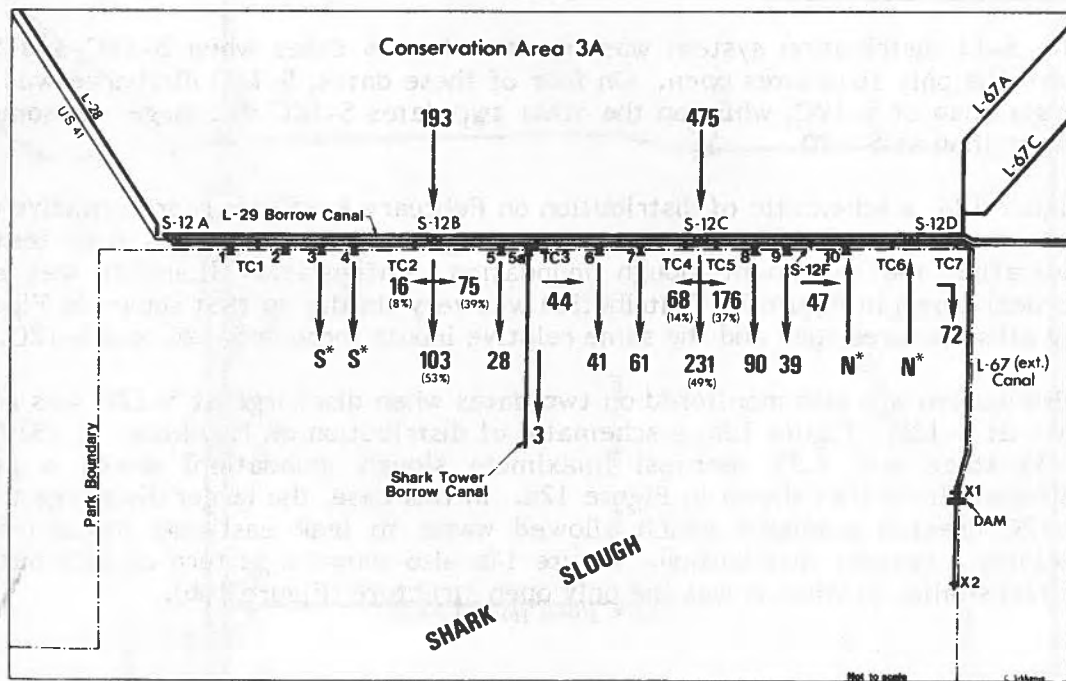
(b). S-12B and S-12C open, September 12, 1979. Asterisk (*) indicates direction of flow when below threshold of current meter.
