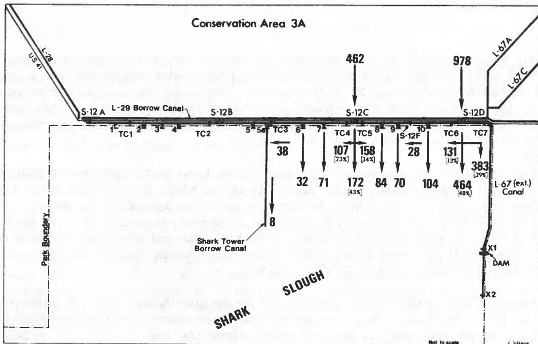
(a) S-12C and S-12D open, larger delivery through S-12D, February 8, 1980.
