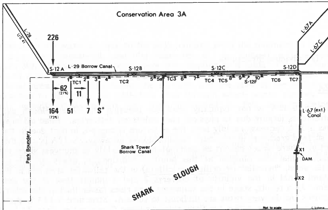
(a) S-12A open, October 3, 1980. Asterisk (*) indicates direction of flow when below threshold of current meter.
