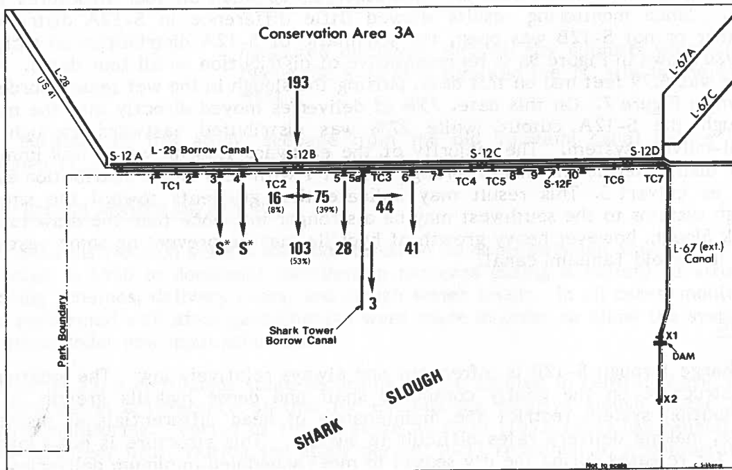
(b) S-12B open, September 12, 1979. Asterisk (*) indicates direction of flow when below threshold of current meter.
