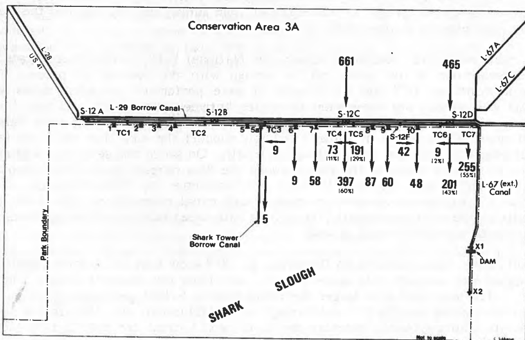
(b). S-12C and S-12D open, larger delivery through S-12C, November 6, 1979.
