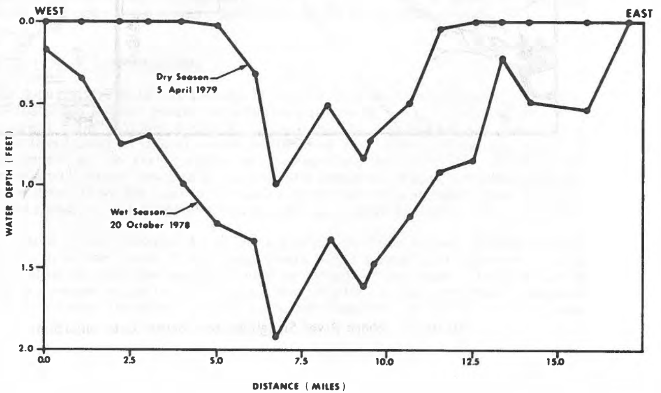
Figure 6. (a) Shark River Slough depth profile monitoring transect. (b) Shark River Slough wet season and dry season depth profiles.
