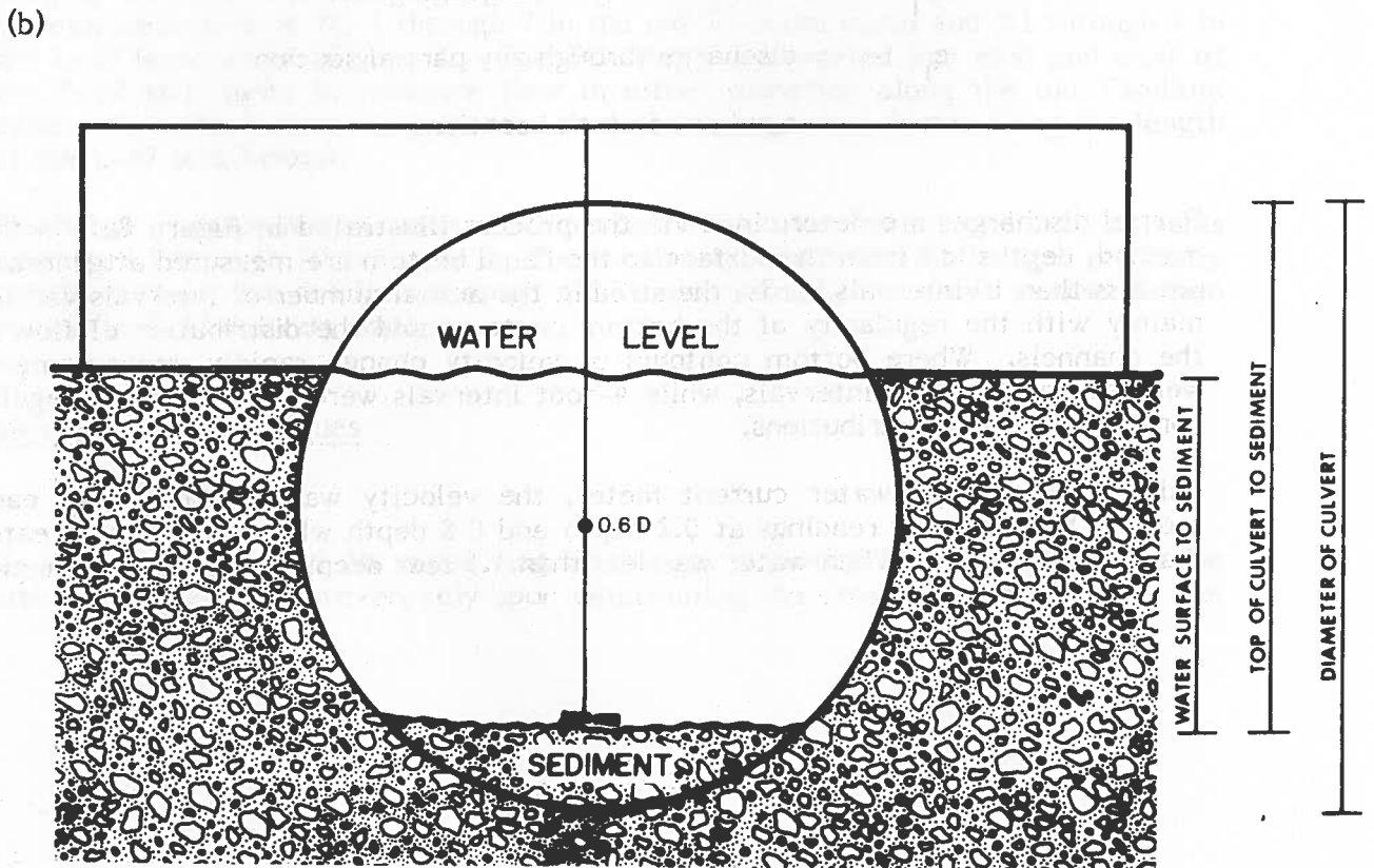
Figure 8. (a) Canal discharge measurement technique. (b) Barrel culvert discharge measurement technique.
