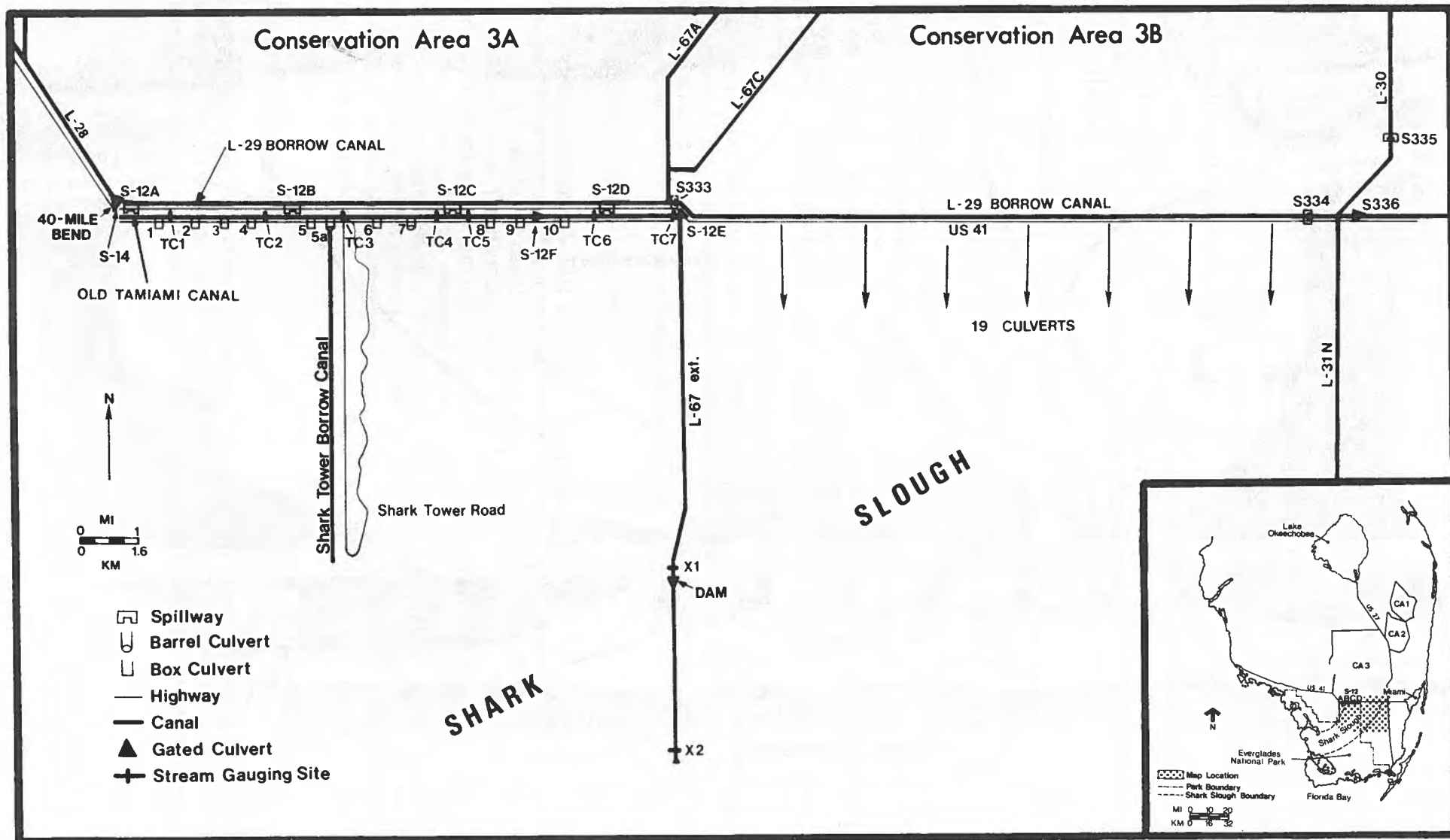
Figure 2. Options for surface water delivery to Shark Slough.
