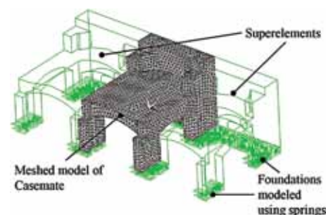
Figure 4: The finite element model of the casemate is built recognizing the elastic constraints of the adjacent casemates as well as the unmodeled foundation.
