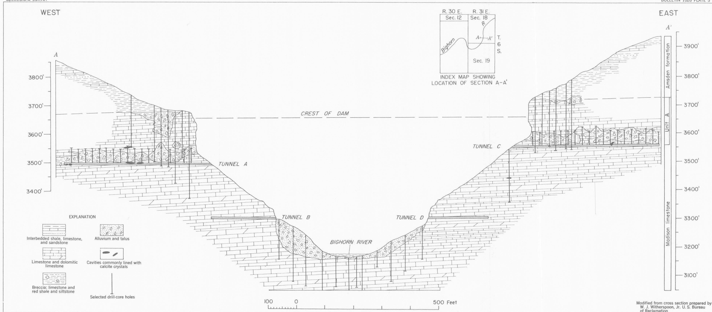
CROSS SECTION OF YELLOWTAIL DAM SITE, MONTANA. DOWNSTREAM VIEW SHOWING BRECCIATION IN UPPER MEMBER (UNIT A) OF THE MADISON LIMESTONE AS INTERPRETED FROM SELECTED DRILL CORES
