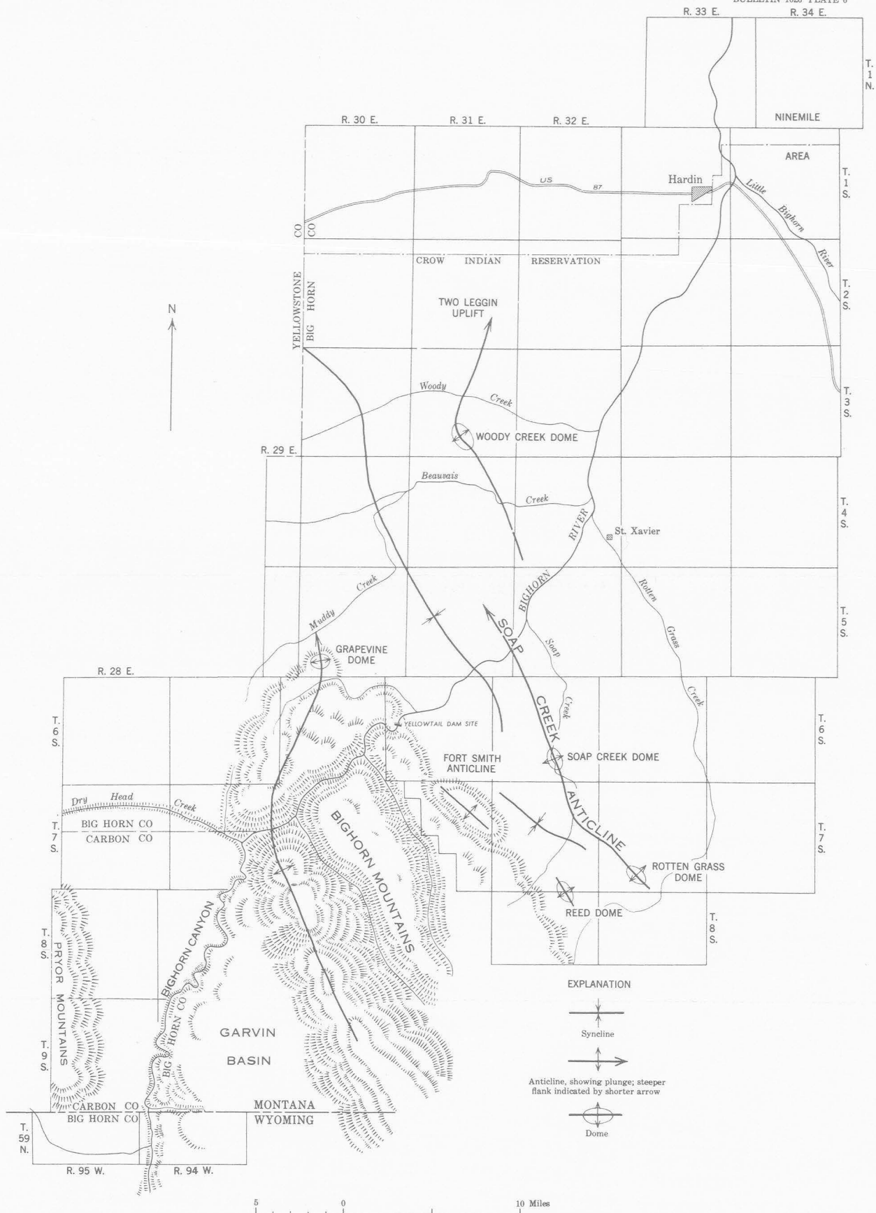
SKETCH MAP OF THE BIGHORN MOUNTAINS AND GREAT PLAINS AREA, MONTANA AND WYOMING, SHOWING MOUNTAINS, BASINS, AND PRINCIPAL AXES OF FOLDING
