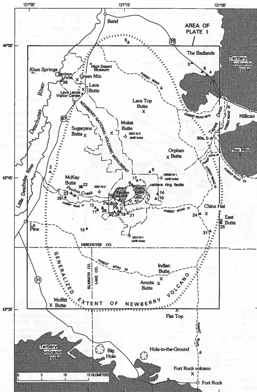
Figure 2. Geographic features in vicinity of map area. Potassium-argon sample locations (triangles) and map numbers shown for samples listed in table 3 except No. 27, which is located 13 km east of Pine Mountain summit. Stipple indicates rocks of known Tertiary age, generalized from Walker and others (1967), Swanson (1969), and MacLeod and Sherrod (1992).
