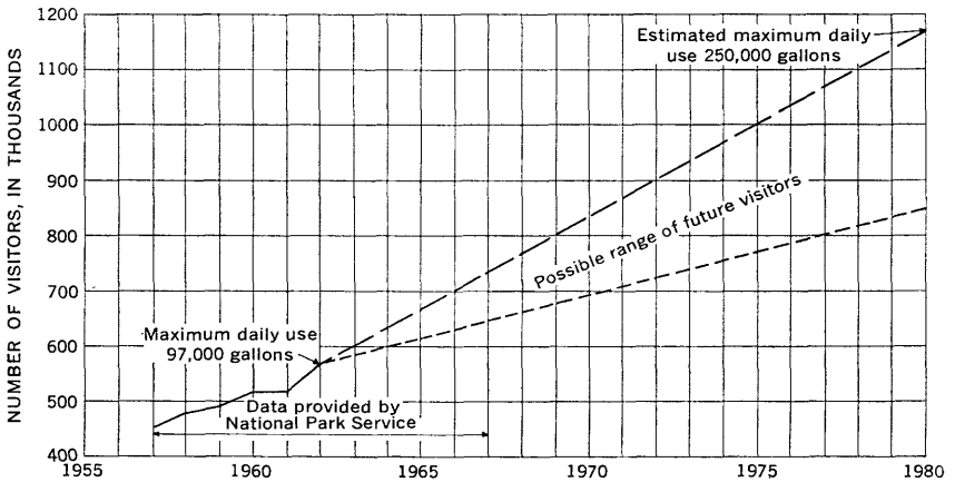
FIGURE 72.—Increasing numbers of visitors and increasing per-capita water use require additional water-supply development for Mammoth Cave National Park.
