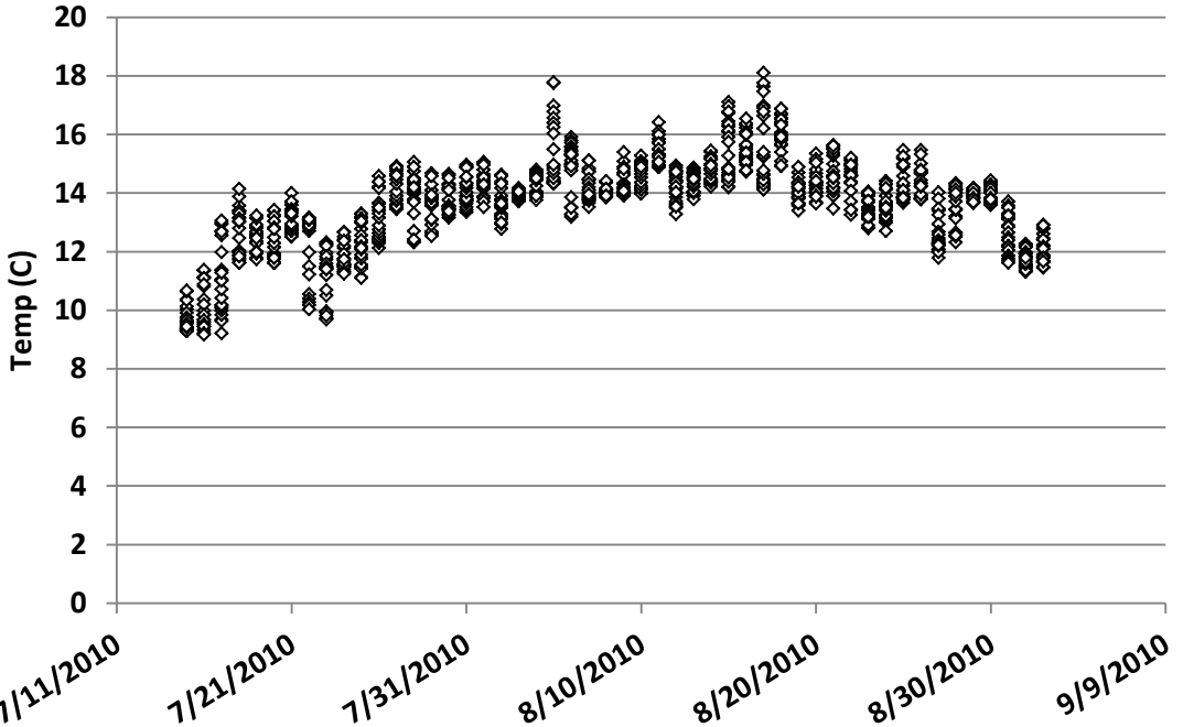
Figure 9. Water temperature measured near the lake bottom in the nearshore zone of St. Mary Lake during 2010.
