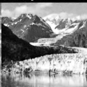
Tidewater glacier
