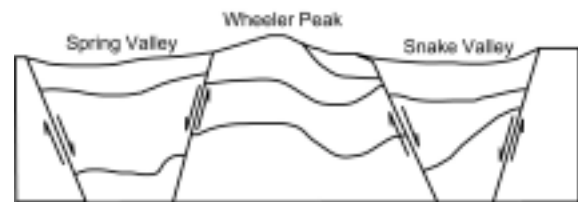
As the earth's crust stretched, faults formed along which valleys down-dropped and mountains uplifted.
