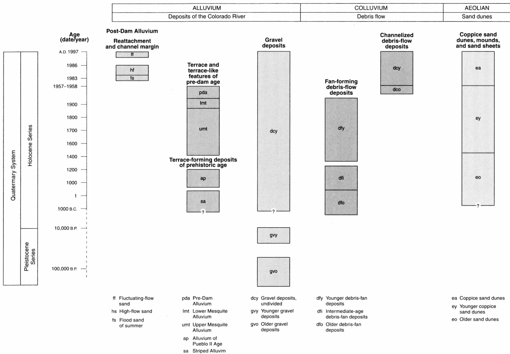
Figure 37. Quaternary deposits in the river corridor correlated with calendar years.
