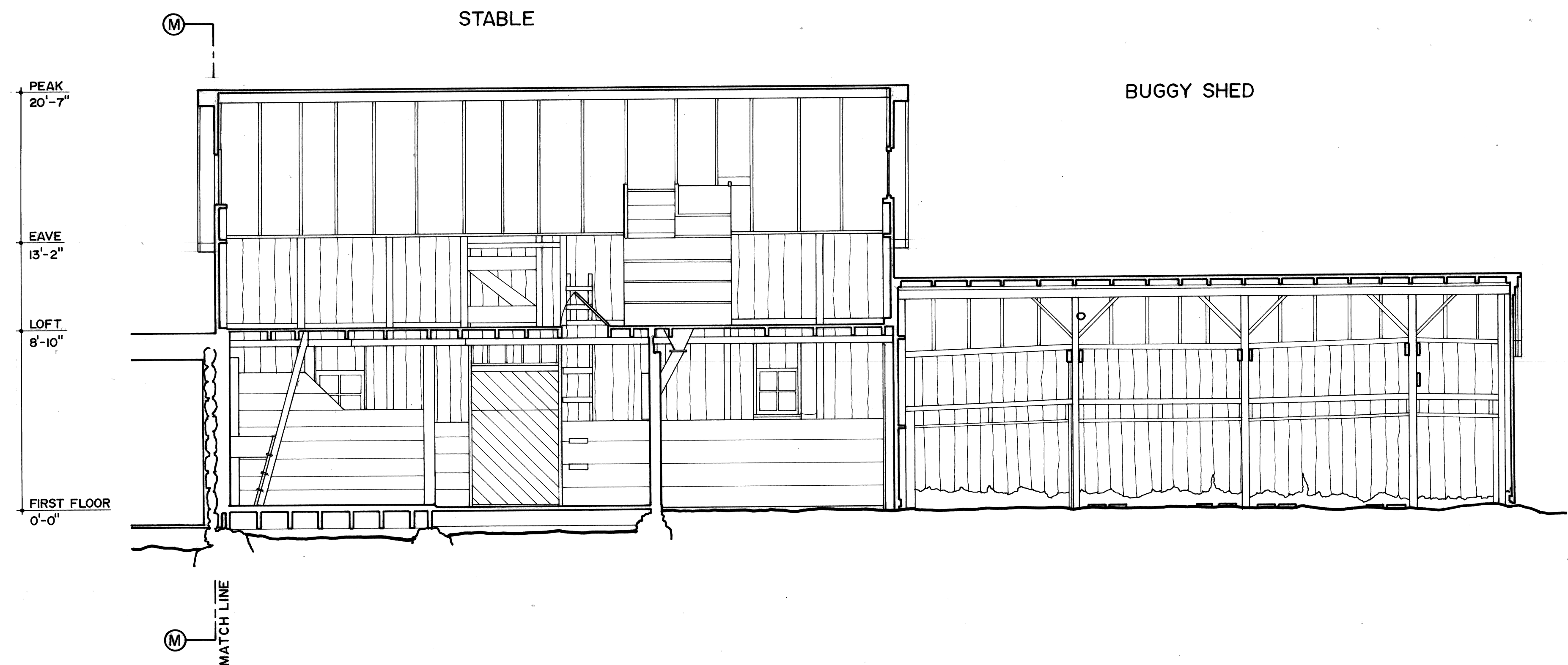
SECTION C-C
