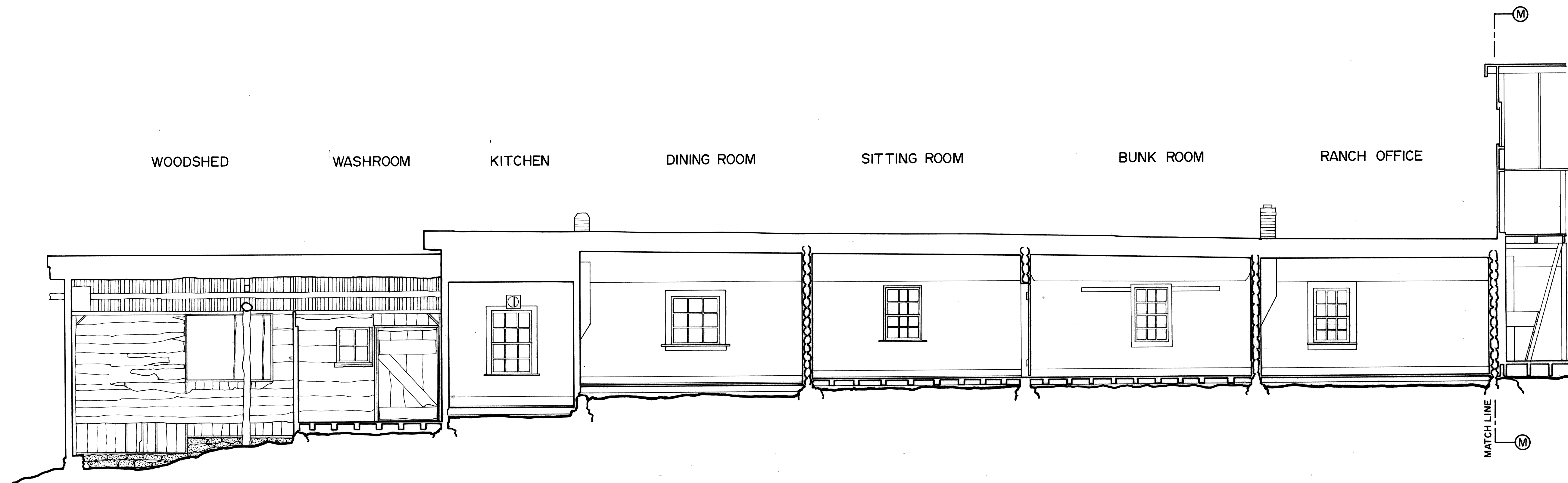
SECTION C-C
