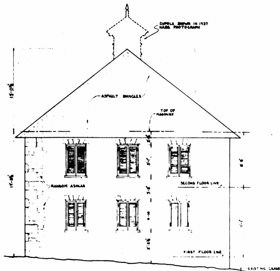
EAST ELEVATION SCALE 1/4" = 1'-0"
