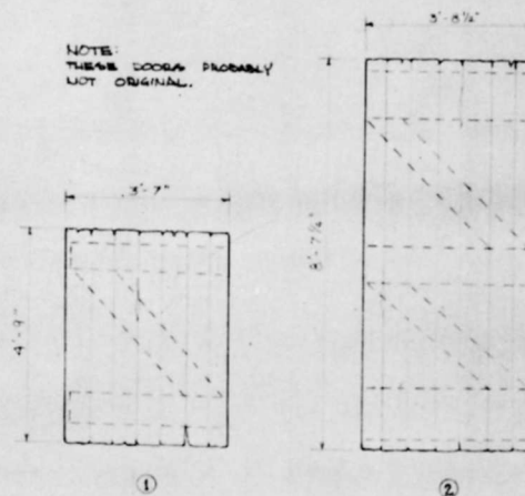
SCALE : 1/2" = 1' - 0"
