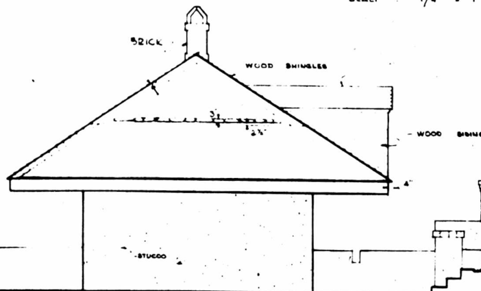
NORTH ELEVATION
