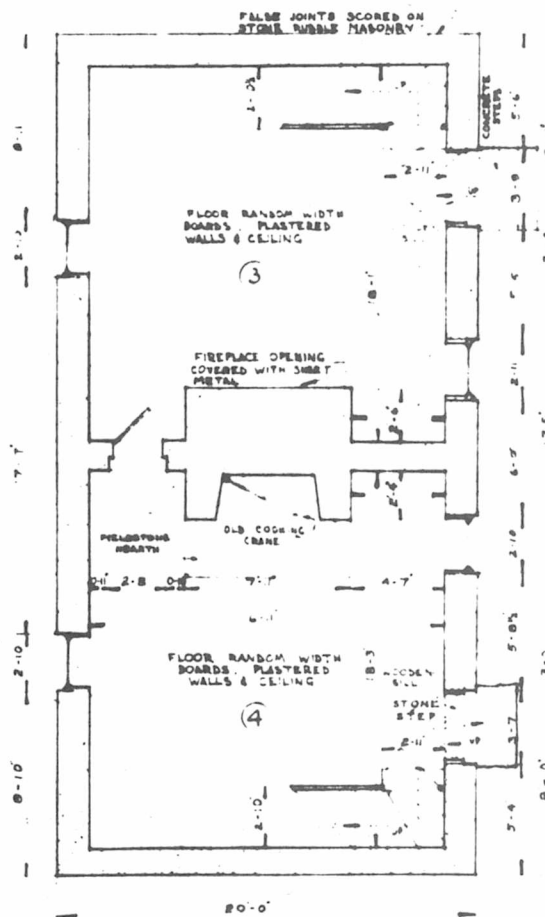
FIRST FLOOR PLAN SCALE: 1/4" = 1'-0"
