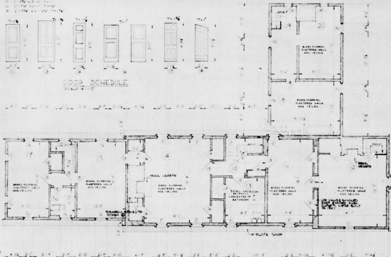
SECOND FLOOR PLAN SCALE: 3/4" = 1'-0"
