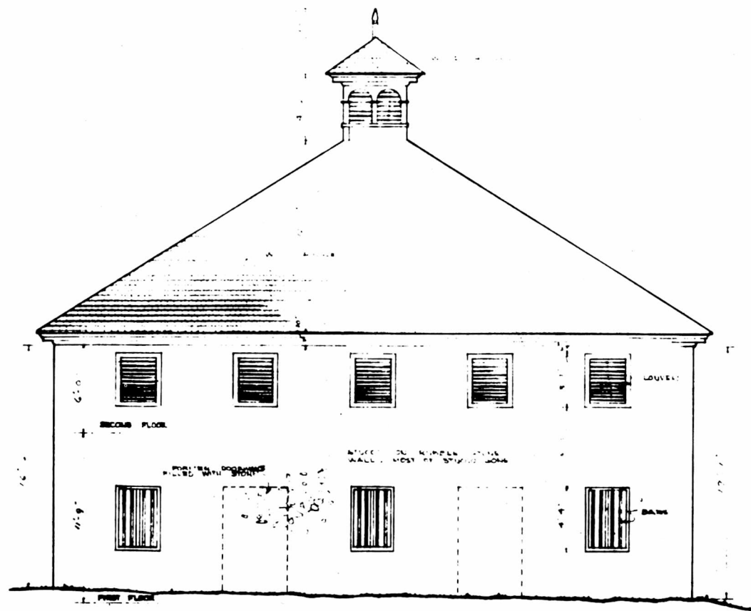
SOUTH ELEVATION
