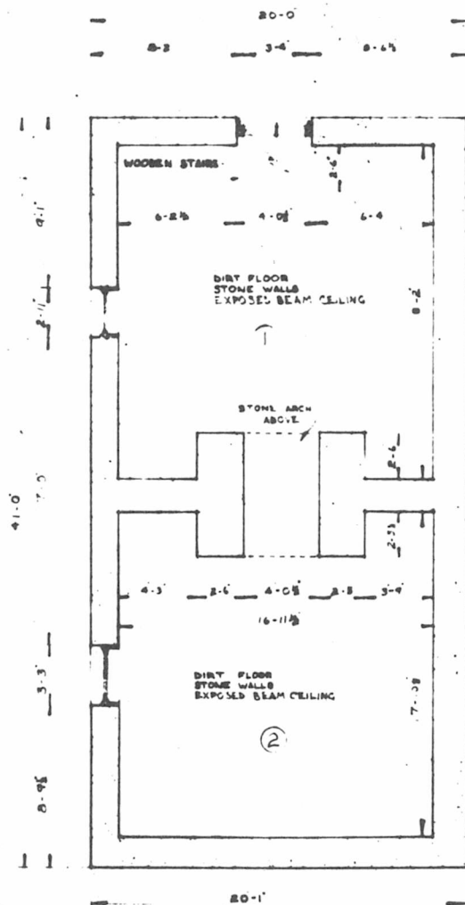
BASEMENT PLAN SCALE: 1/4" = 1'-0"
