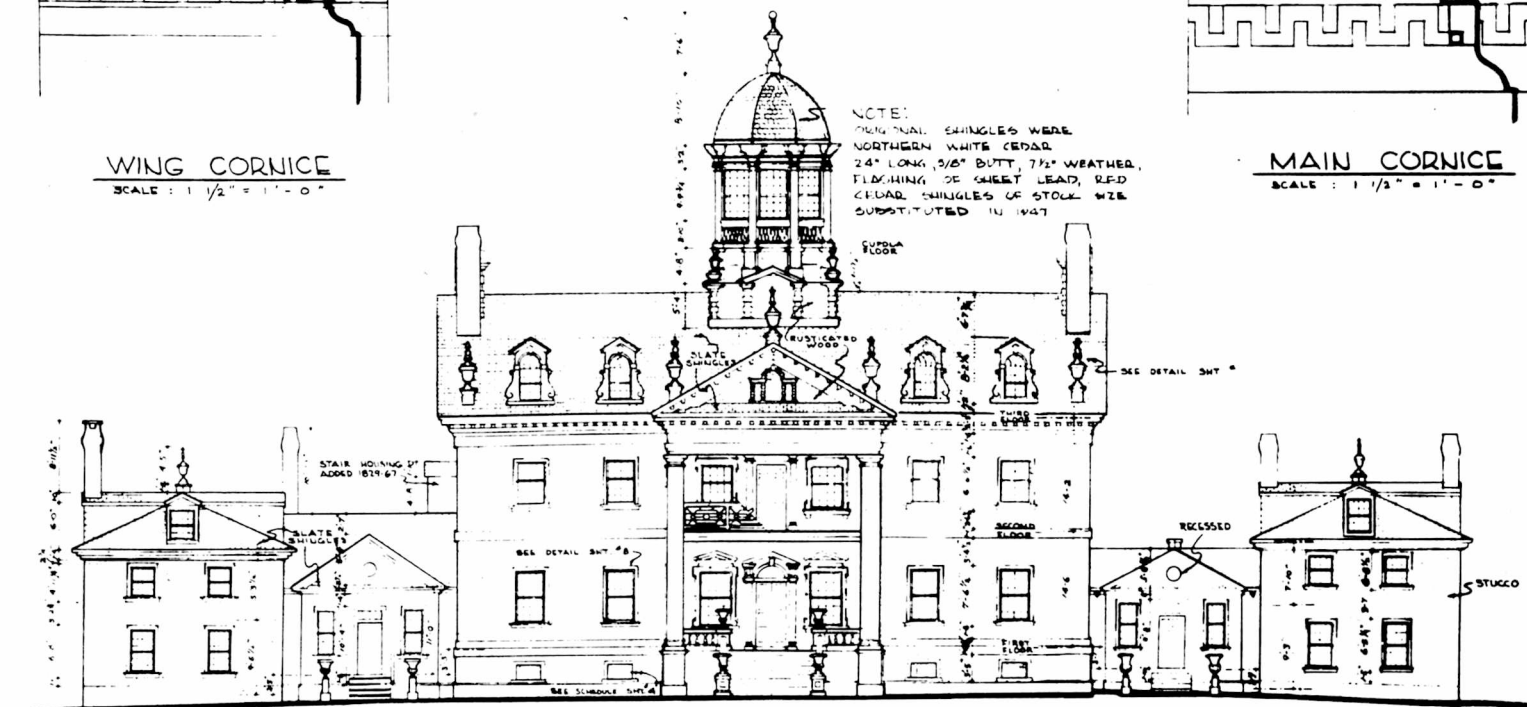
NORTH ELEVATION
