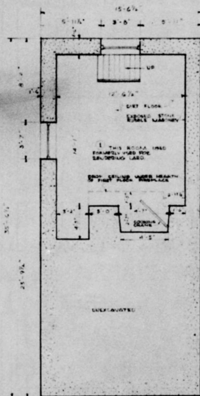
BASEMENT
