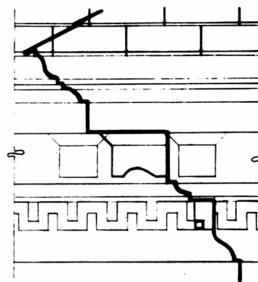
MAIN CORNICE
