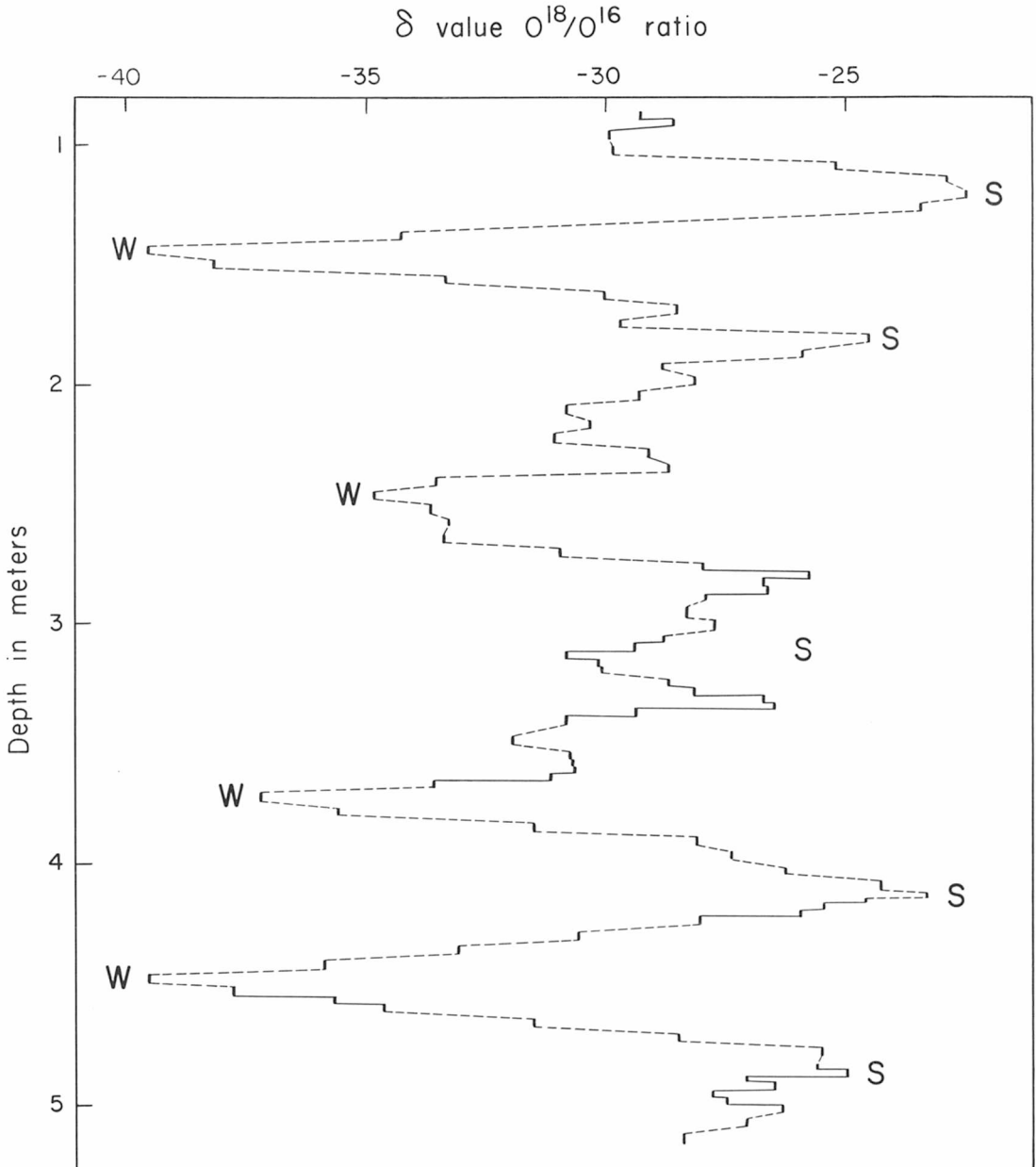
FIGURE 23. Seasonal variations in the O^{18}/O^{16} ratio can be used to identify annual layers in accumulated firn on Greenland Ice Sheet. S=summer layer; W=winter layer, data from Epstein and Benson, on basis of samples supplied by Snow, Ice, Permafrost Research Establishment.
