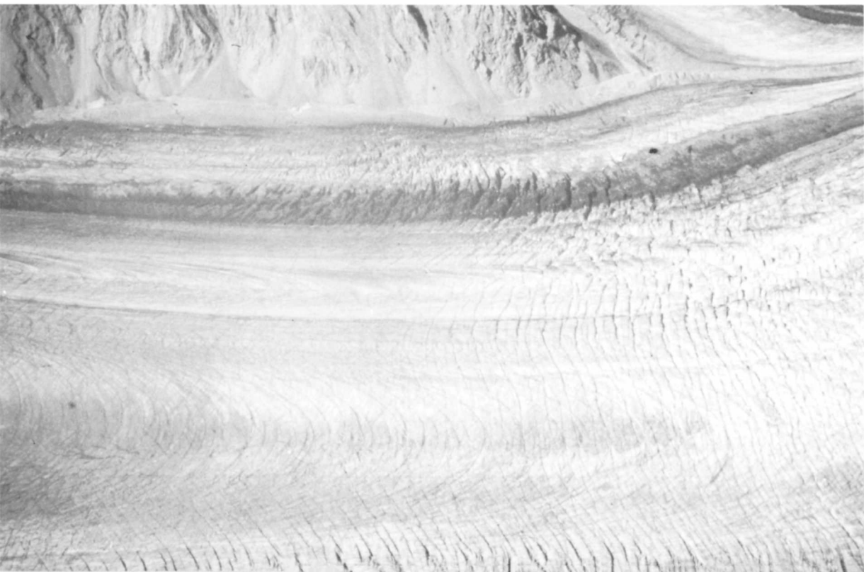
B —Air view of valley glacier in Yakutat Range east of Yakutat, Alaska. Note the double arcuate pattern of foliation visible in the two central ice streams. Late August, 1951.
