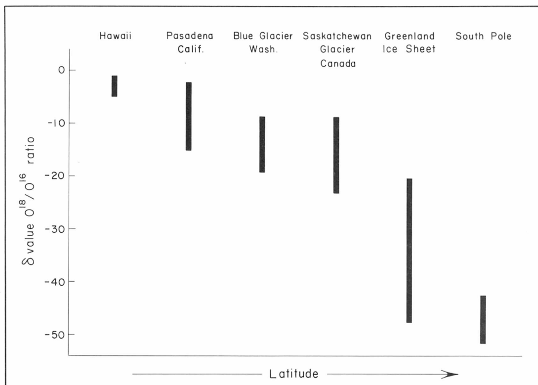
FIGURE 21. Plot showing that O^{18}/O^{16} ratio of precipitation becomes more negative with higher latitude.
