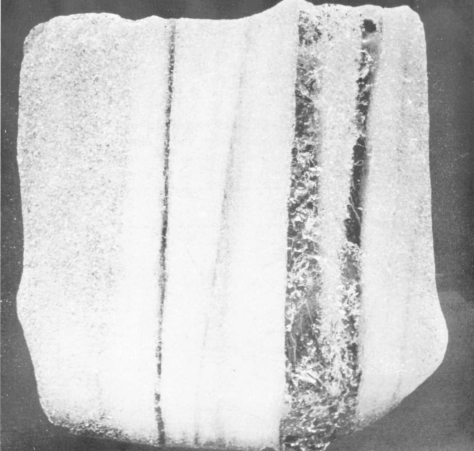
A —Close-up view of foliation in a block of ice about 12 inches across. Dark bands are clear ice, white bands in middle are fine ice, less whitish bands at outer edges are composed of coarse-bubbly ice.
