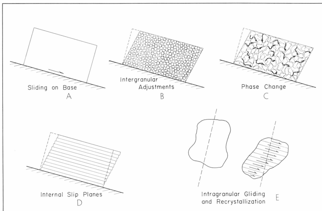
FIGURE 15. Sketches illustrating various possible mechanisms of glacier movement.
