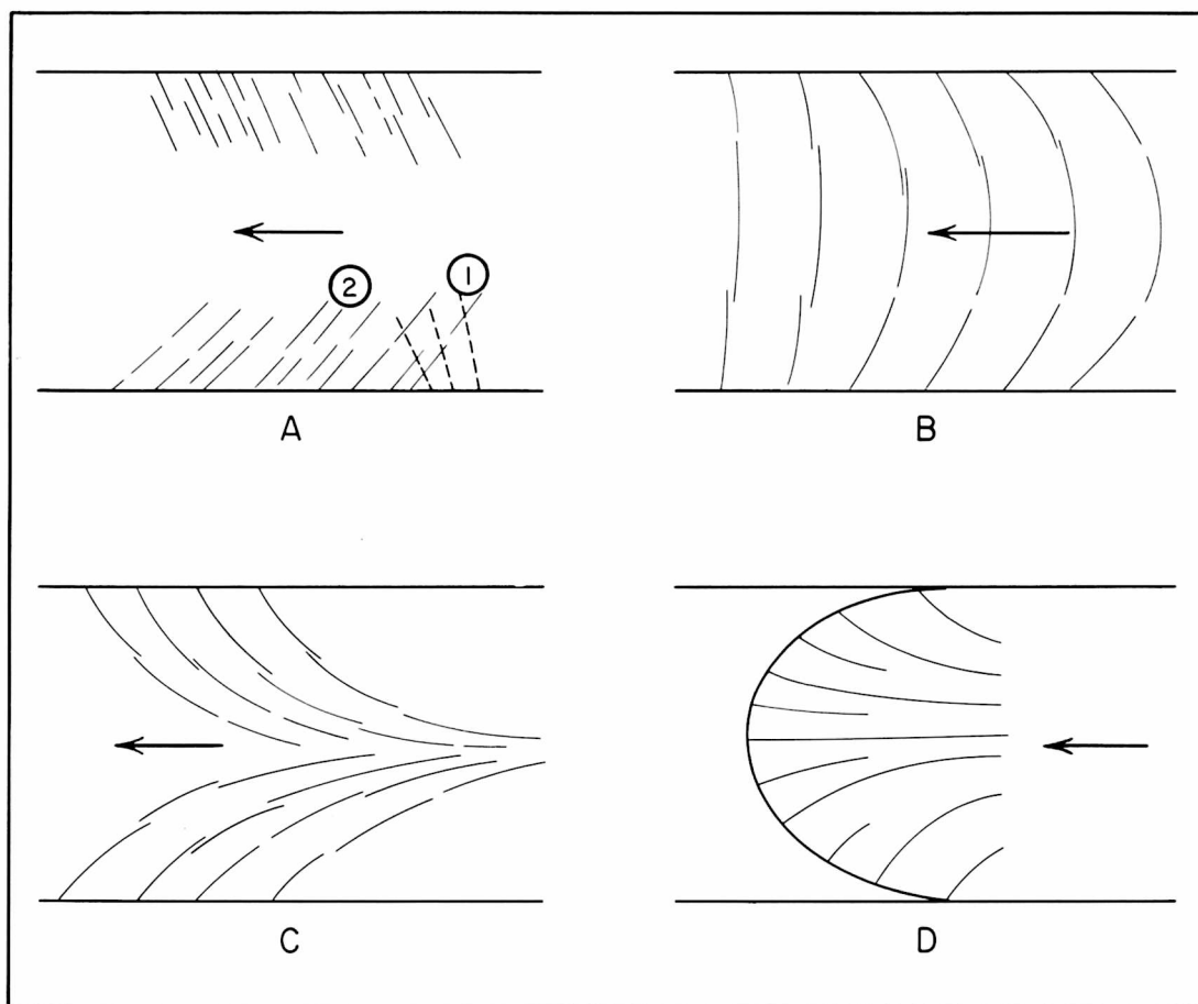
FIGURE 16. Principal types of crevasses in valley glaciers. A—Marginal, 1) old rotated crevasses, 2) newly formed crevasses; B—Transverse; C—Splaying; D—Radial splaying. Arrow indicates flow direction.
