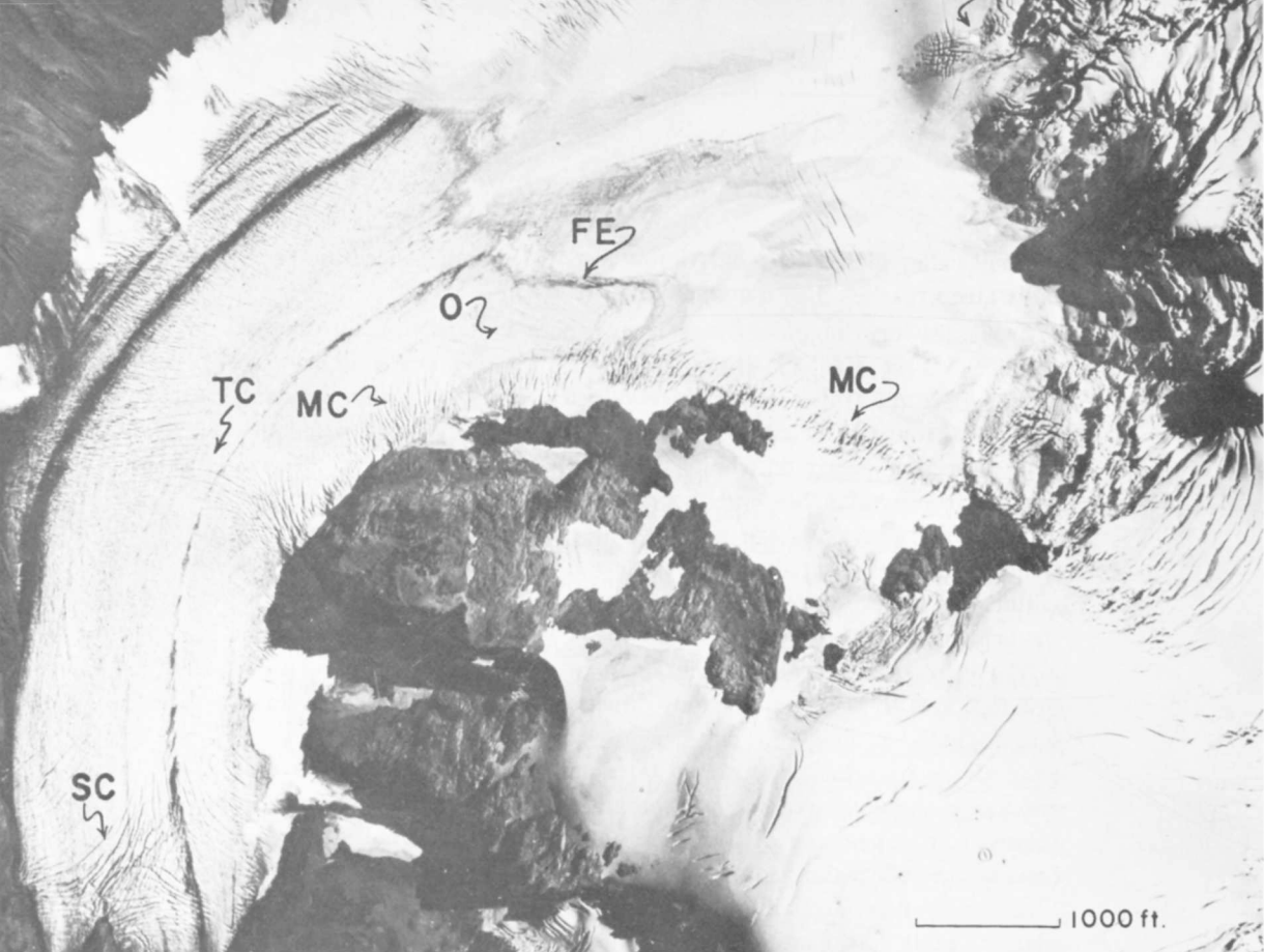
A —Vertical air photo of Blue Glacier showing splaying crevasses (SC) near terminus, transverse crevasses (TC) in middle reach, marginal crevasses (MC), and ticktacktoe crevasse pattern (TTC). Also shown are the firn edge (FE), faint ogives (O), and the icefall at the right margin of the photo. September 11, 1957.
