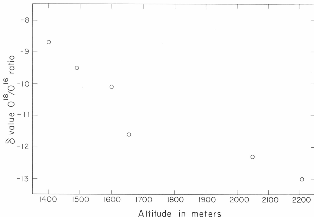
FIGURE 22. Plot of O^{18}/O^{16} ratios in snow from Blue Glacier showing that ratios become more negative with increasing altitude at rate of about 1 unit per 650 feet elevation.
