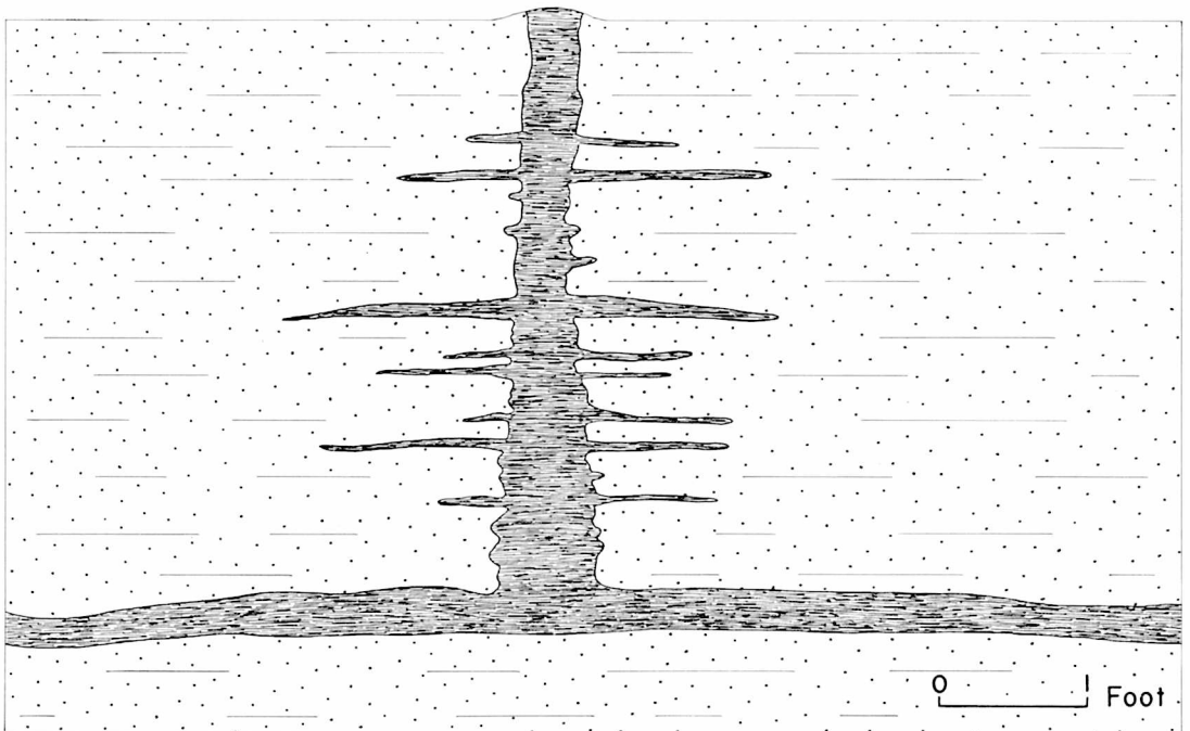
FIGURE 6. Field sketch of a pipe-like mass of ice with horizontal projections formed in firn of upper Seward Glacier by refreezing of downward percolating meltwater.
