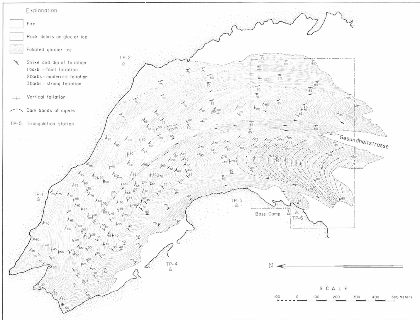
Figure 19. Structures exposed on surface of Blue Glacier below the firn edge as mapped in summer of 1959.
