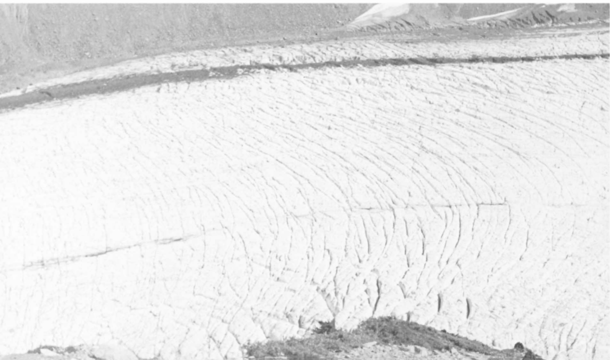
B —Transverse crevasses in lower Blue Glacier, Olympic Mountains, Washington, as viewed from west valley wall in August, 1958. Glacier flows to left and initial concavity of crevasse traces is partly straightened out downvalley by differential flow.
