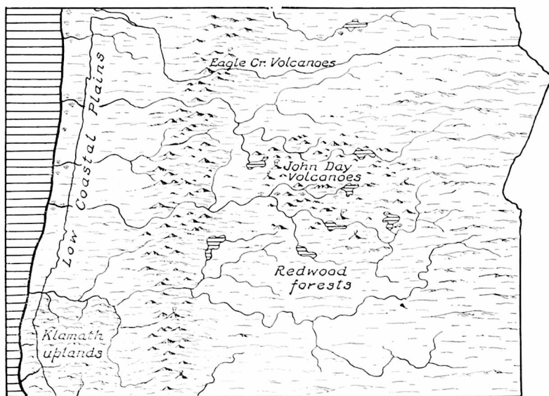
Fig. 3. Early Miocene (late John Day). Volcanoes active throughout the length of the ancestral Cascades and in the John Day region.
