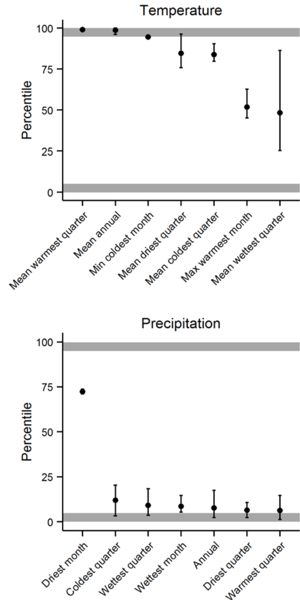
Figure 2. Recent temperature and precipitation percentiles at Organ Pipe Cactus National Monument (including areas within 30-km [18.6-mi] of the park’s boundary). Black dots indicate average recent percentiles across the 10, 20, and 30-year intervals (moving windows). Variables are considered “extreme” if the mean percentiles are <5 th percentile or >95 th percentile (i.e., the gray zones, where recent climate is pushing the limits of all observed climates since the year 1901). Black bars indicate the range of recent percentiles across 10, 20, and 30-year moving windows (larger bars indicate higher sensitivity to moving window size).
