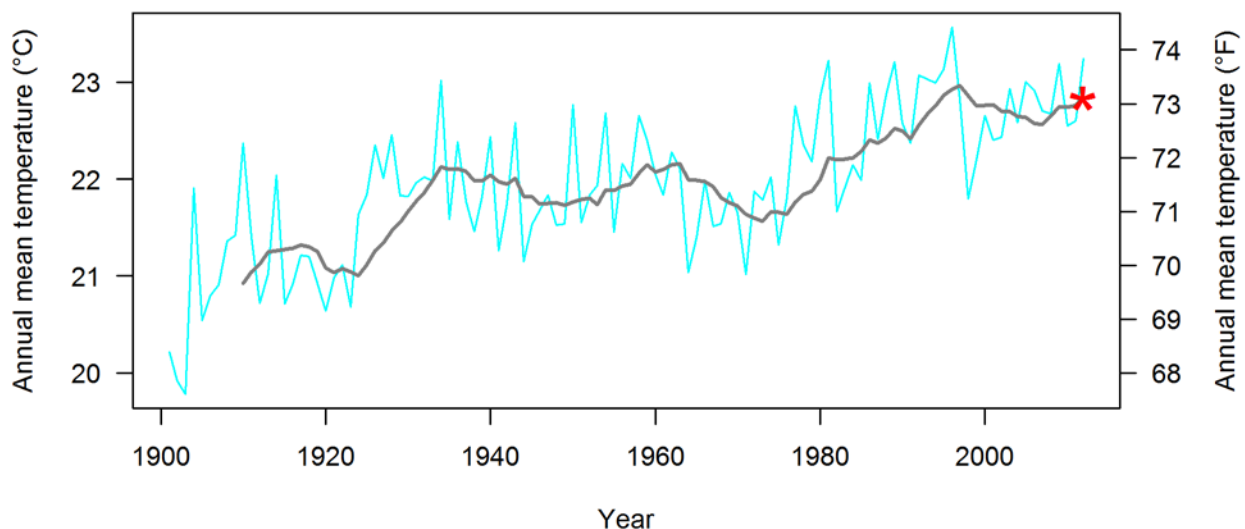
Figure 1. Time series used to characterize the historical range of variability and most recent percentile for annual mean temperature at Organ Pipe Cactus National Monument (including areas within 30-km [18.6-mi] of the park’s boundary). The blue line shows temperature for each year, the gray line shows temperature averaged over progressive 10-year intervals (10-year moving windows), and the red asterisk shows the average temperature of the most recent 10-year moving window (2003–2012). The most recent percentile is calculated as the percentage of values on the gray line that fall below the red asterisk (see results of most recent percentiles for all temperature and precipitation variables in Figure 2).
