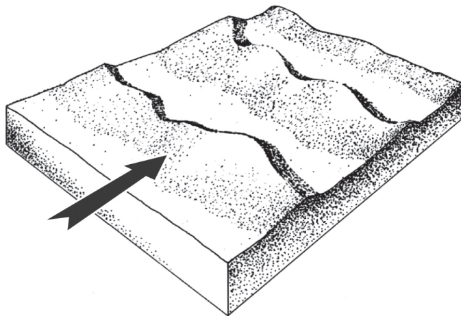
BARCHANOID RIDGE. Arrow shows prevailing wind direction.
