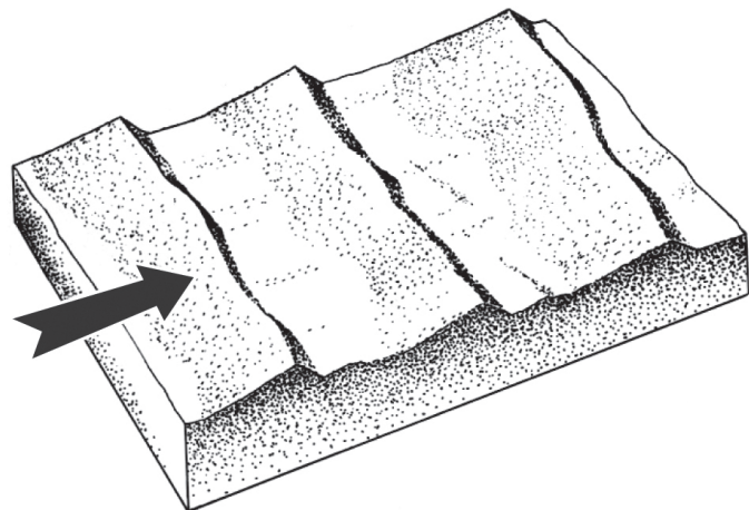
TRANSVERSE DUNE. Arrow shows prevailing wind direction.
