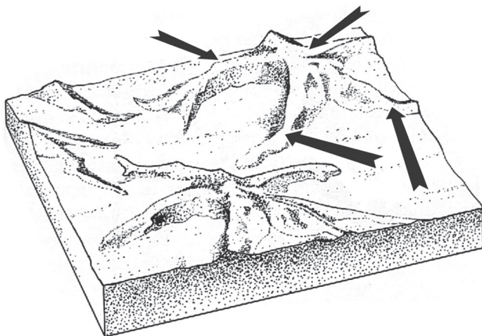
STAR DUNES. Arrows show effective wind directions.
