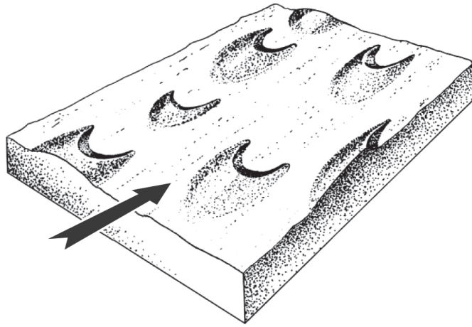
BARCHAN DUNES. Arrow shows prevailing wind direction.
