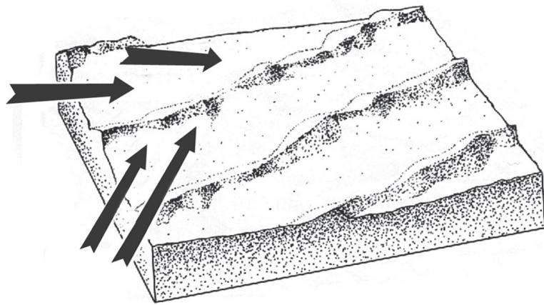
LINEAR DUNES. Arrows show probable dominant winds.
