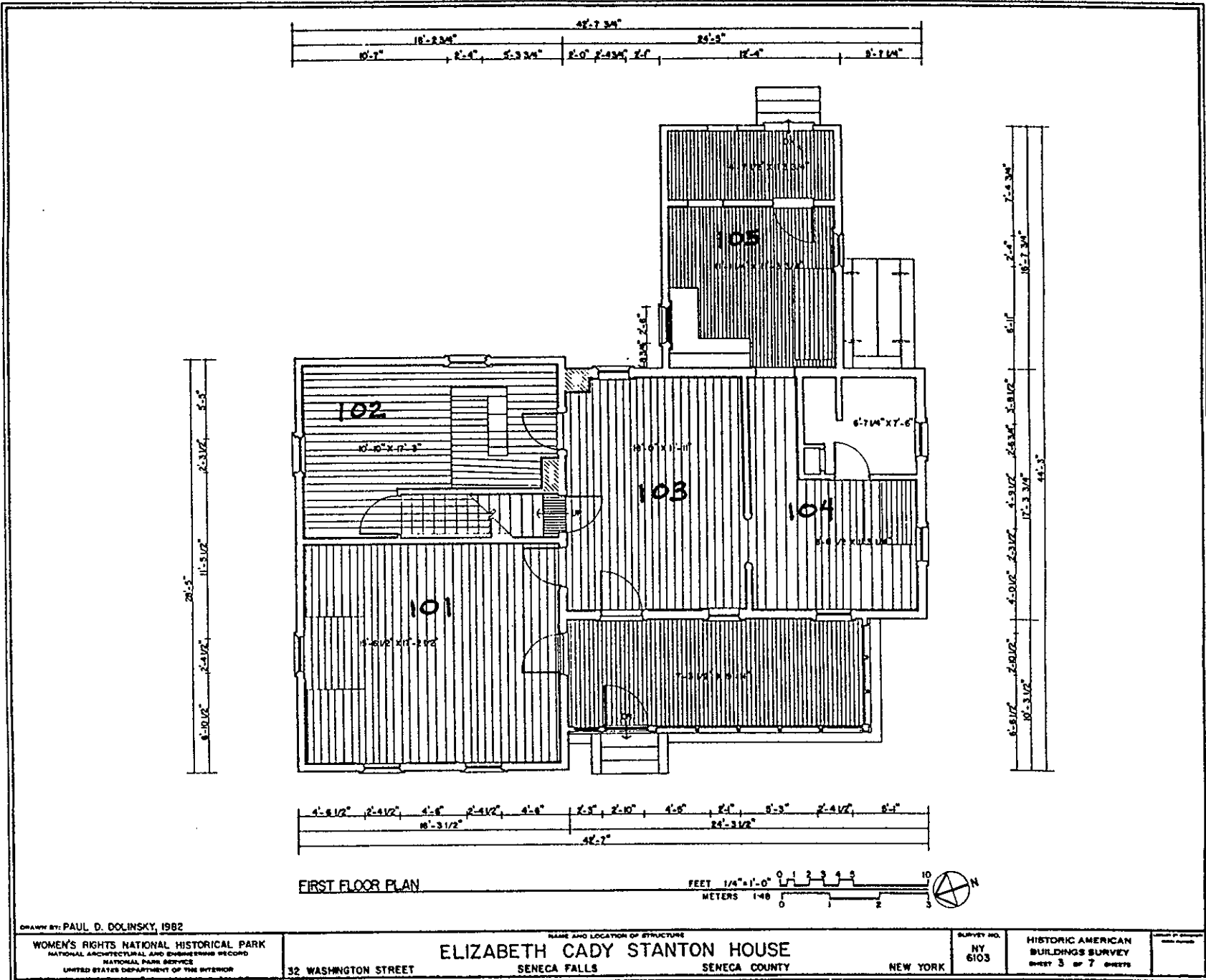
Figure 35. Stanton House: first-floor plan, summer 1982.
