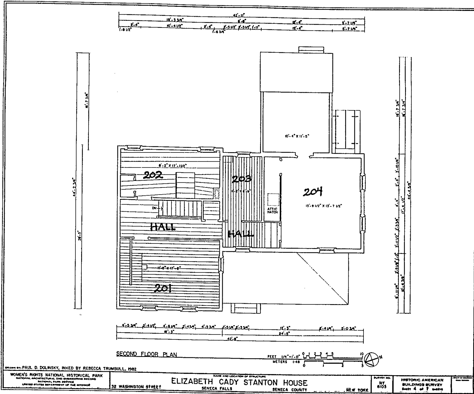
Figure 55. Stanton House: second-floor plan, summer 1982.
