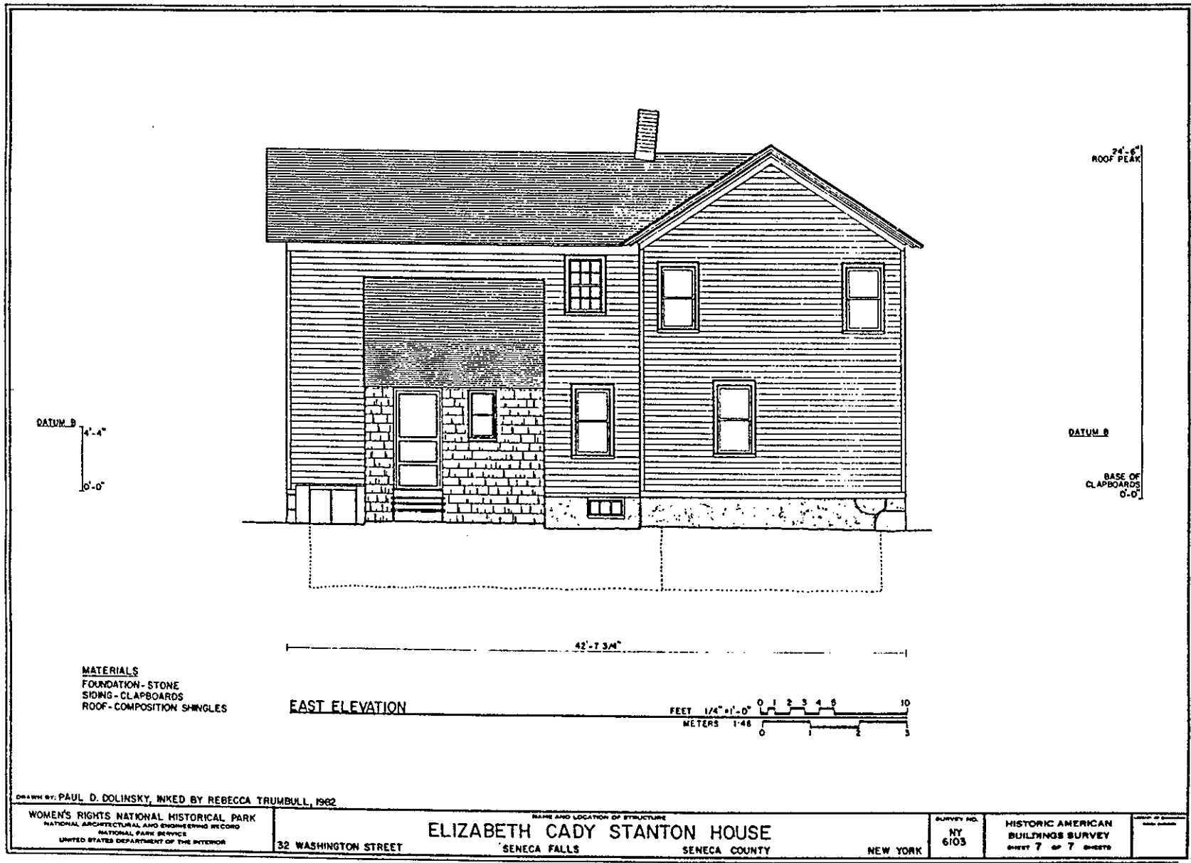
Figure 29. Stanton House: east elevation, summer 1982.
