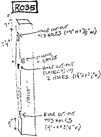
6 3/4" H x 3/4" W x 1" THICK LEFT SIDE ARCHITRAVE
