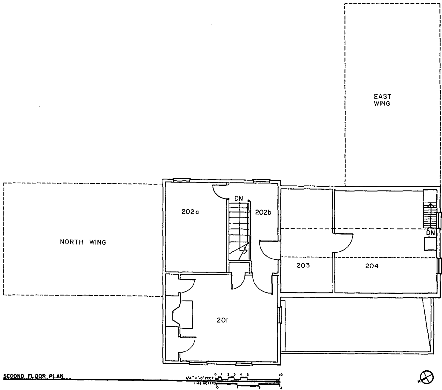
Figure 17. Conjectural second-floor plan of William Bayard's house, circa 1837.
