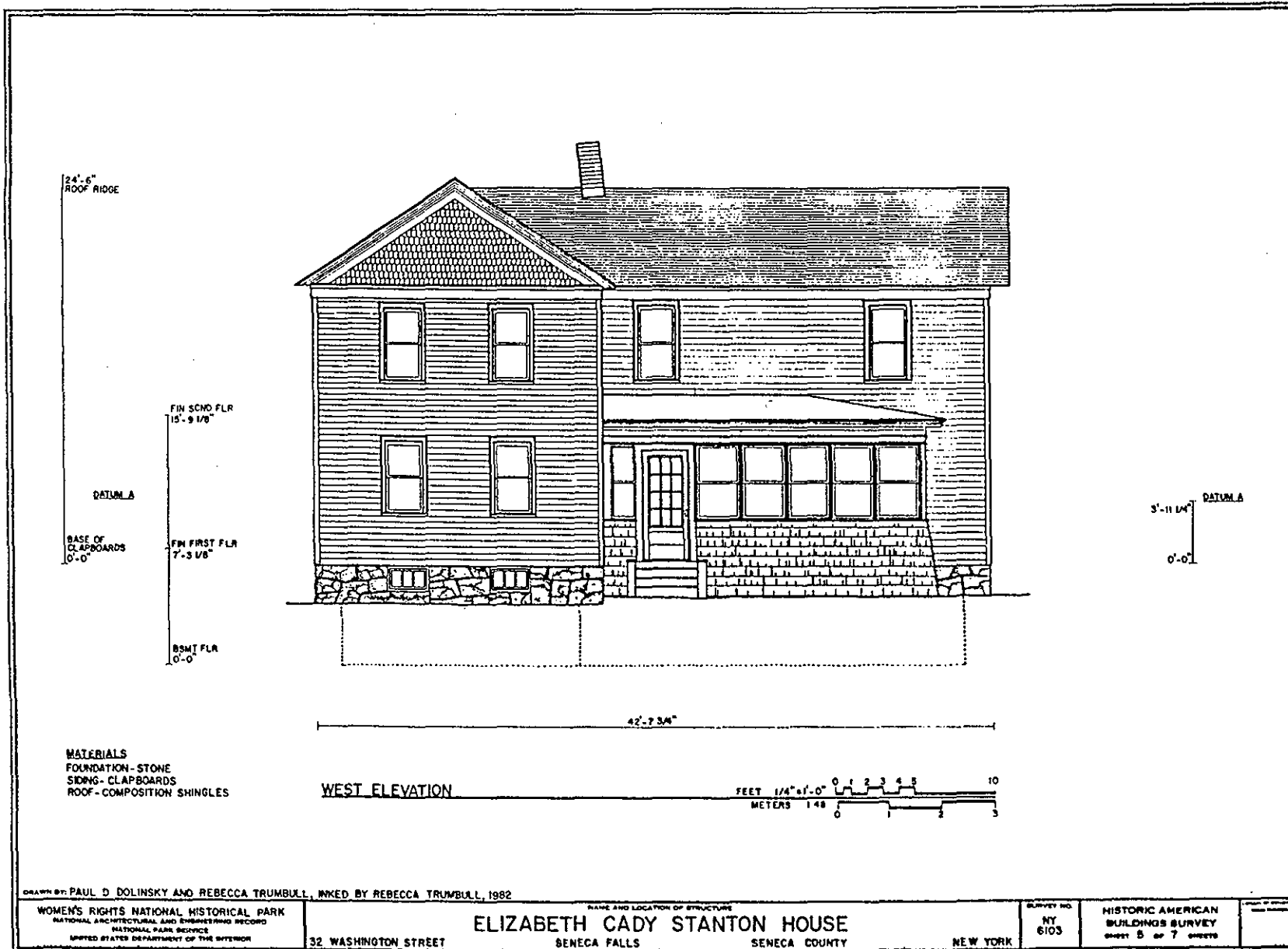
Figure 25. Stanton House: west elevation, summer 1982.
