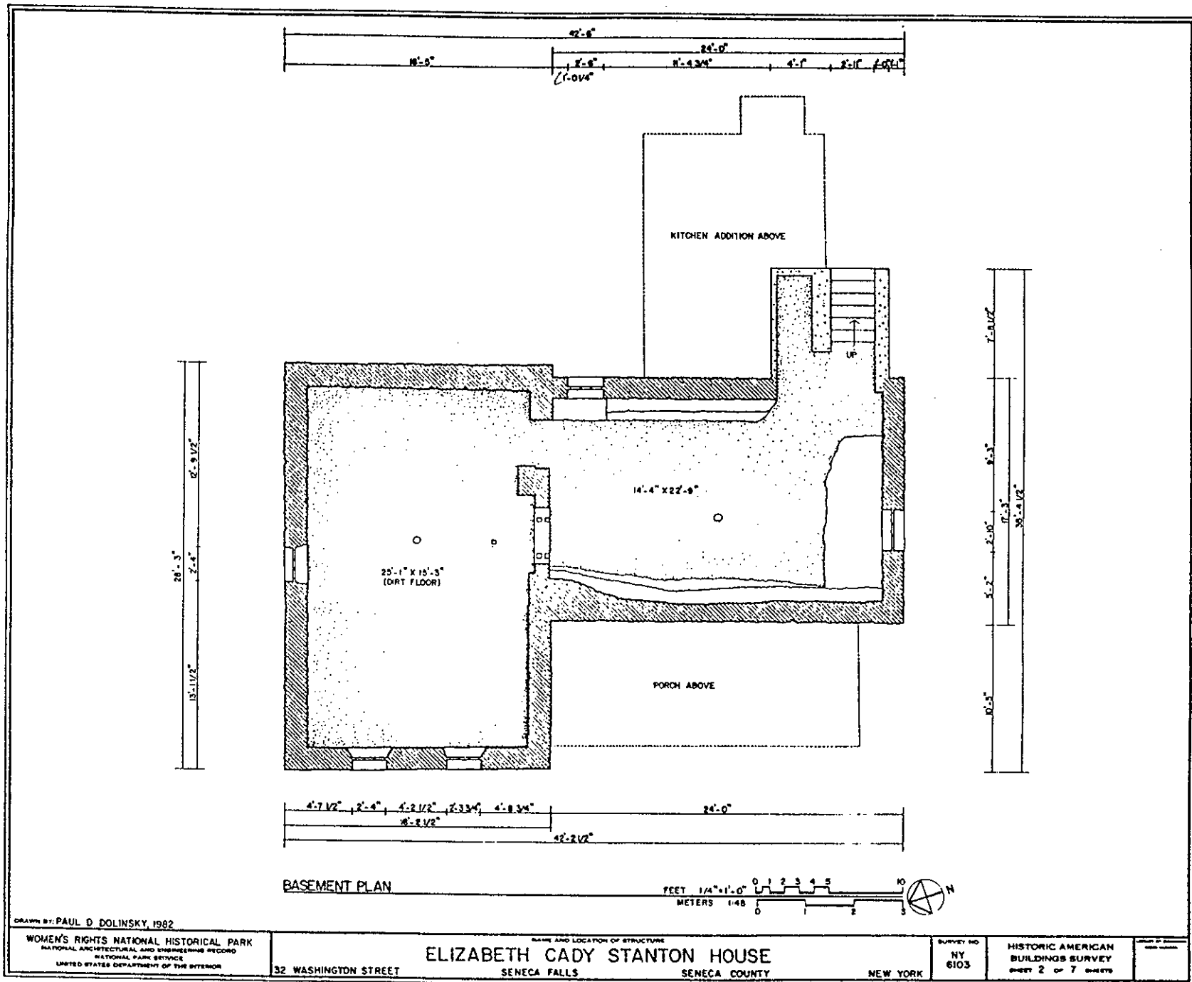
Figure 34. Stanton House: basement [cellar] plan, summer 1982.
