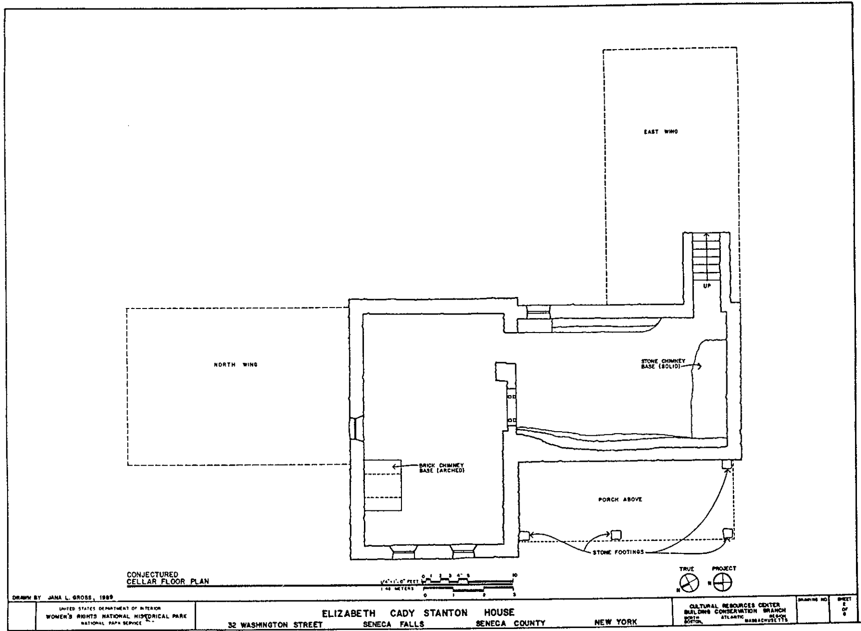
Figure 22. Stanton House: Conjectural cellar plan, circa 1847-62.
