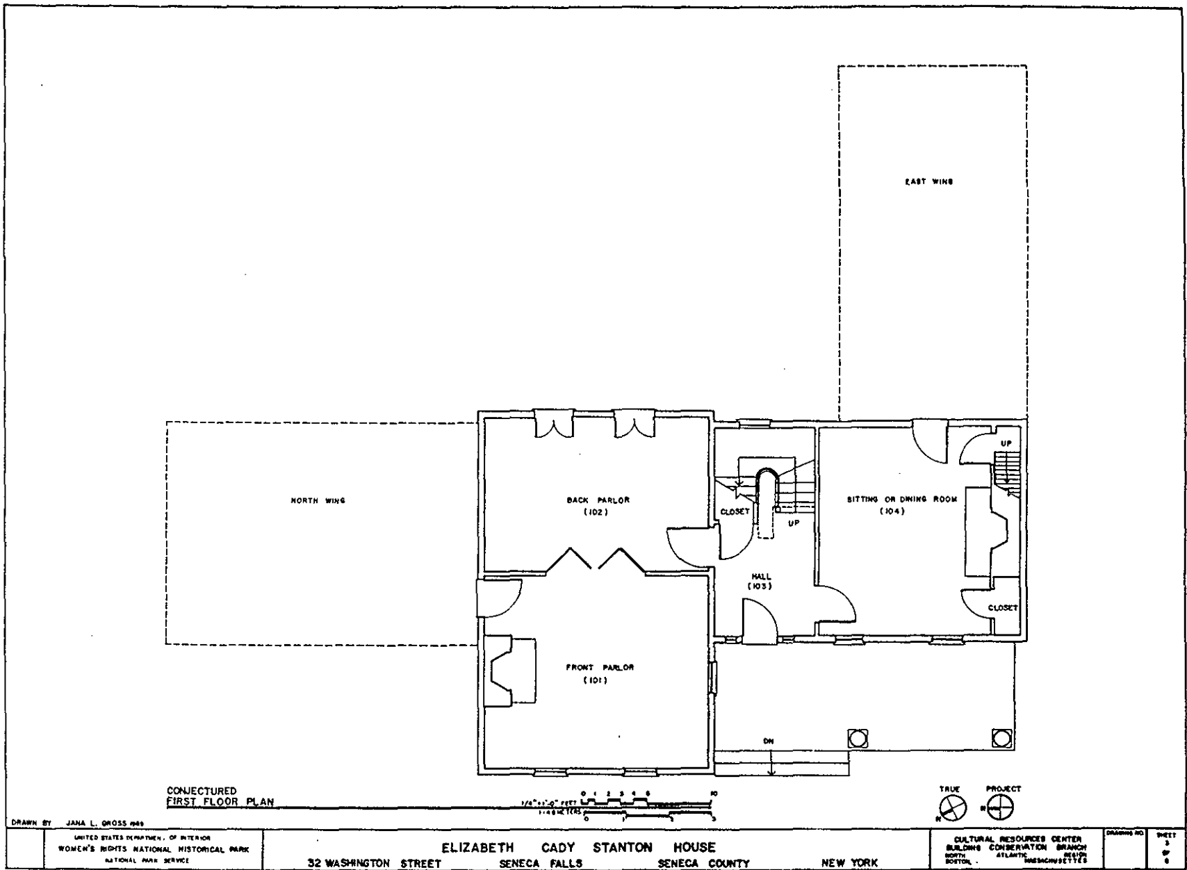
Figure 23. Stanton House: conjectured first-floor plan, circa 1847-62.
