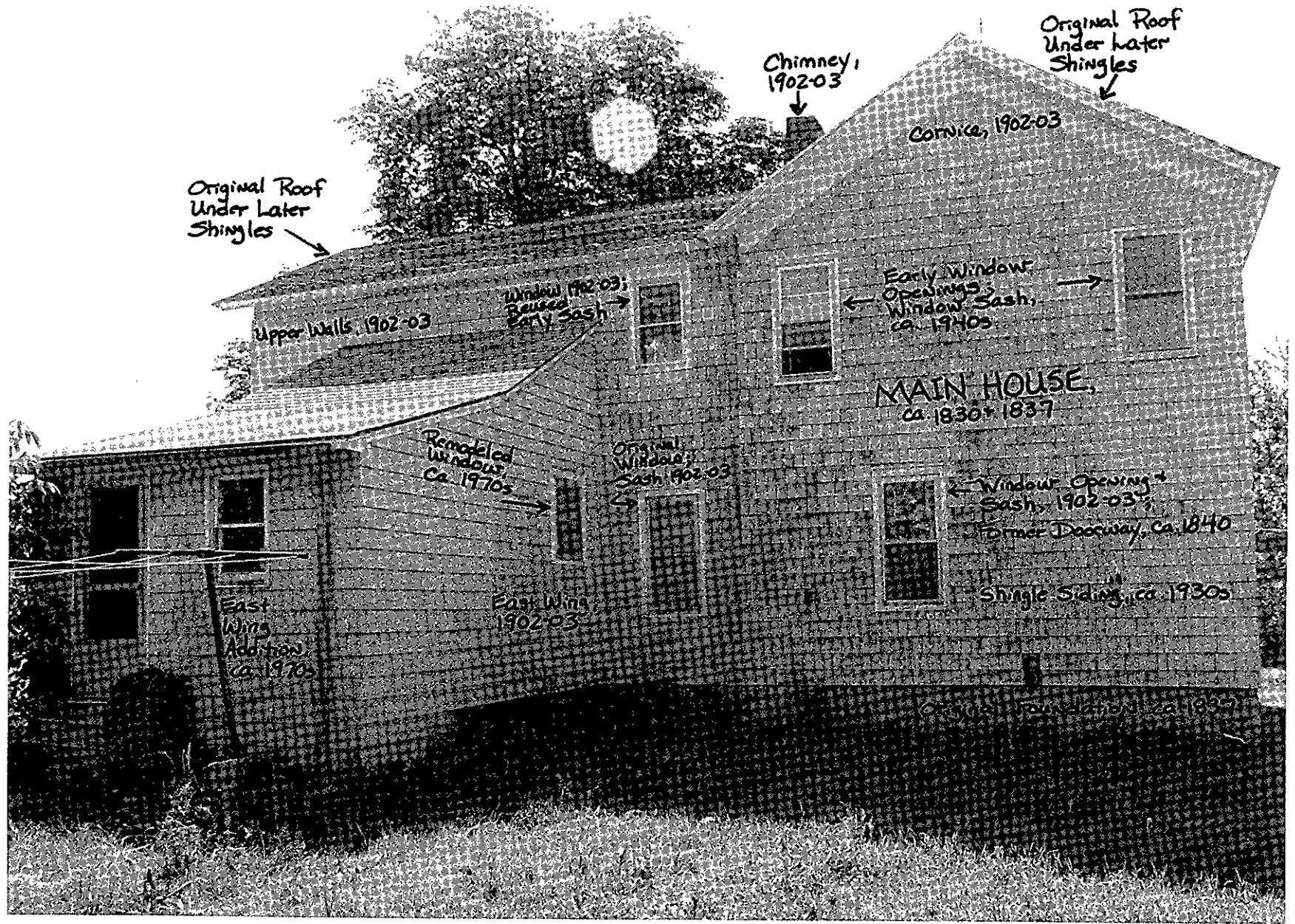
Figure 31. Stanton House: east elevation, June 1982.
