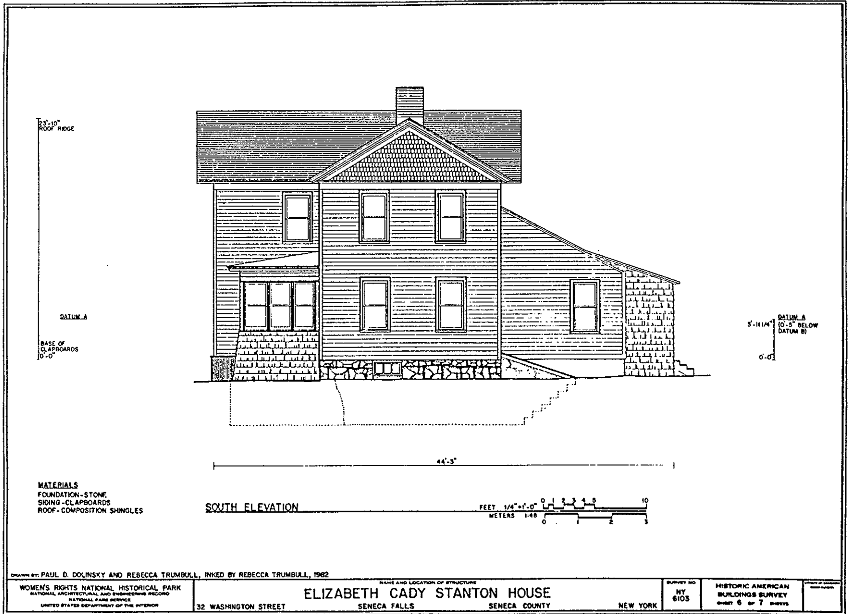
Figure 28. Stanton House: south elevation, summer 1982.
