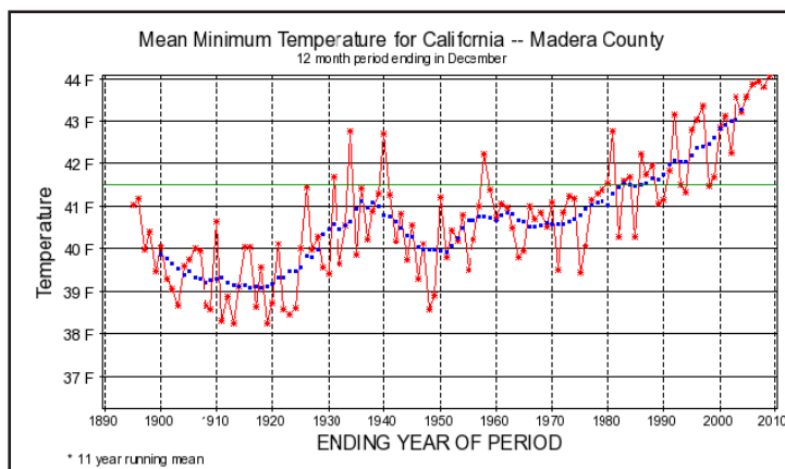
Figure 1. Madera County (Yosemite region) mean calendar year minimum temperature (1895–2009). Red: individual years. Blue: 11-year running mean. Green: 1971–2000 mean. Data from PRISM. Source: Interactive plots, WRCC/UArizona Westmap (from Edwards and Redmond 2011).
